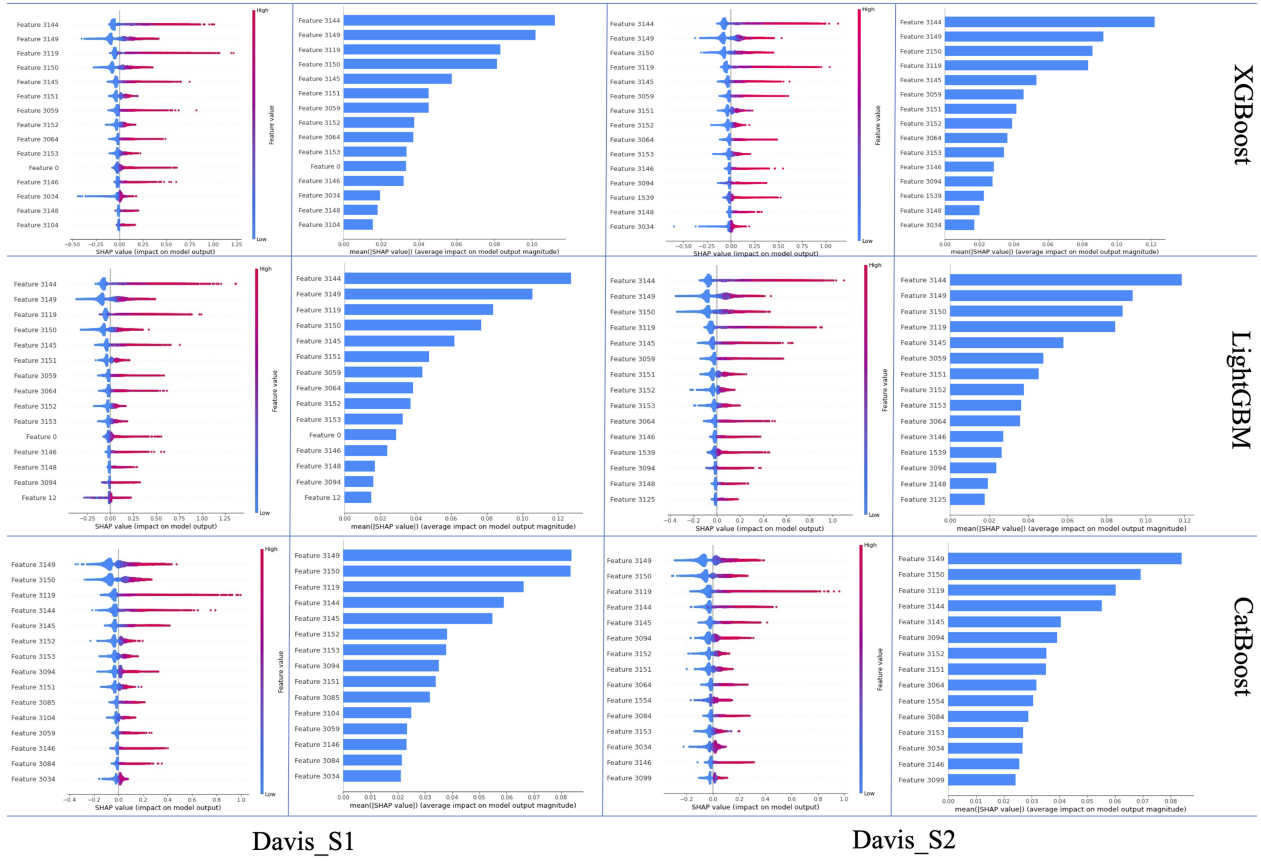
Figure 4. The top 20 features of regression tree-based feature selection methods for Davis.
