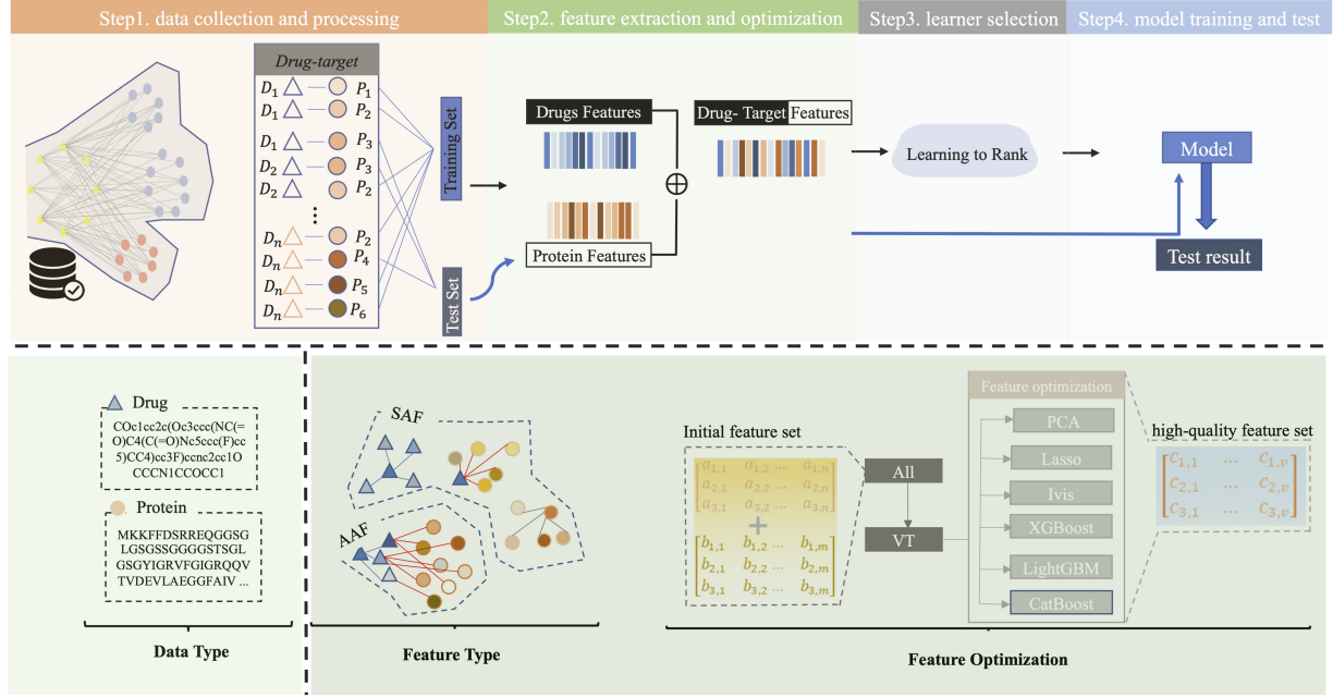
Figure 1. The overall architecture of this study.
