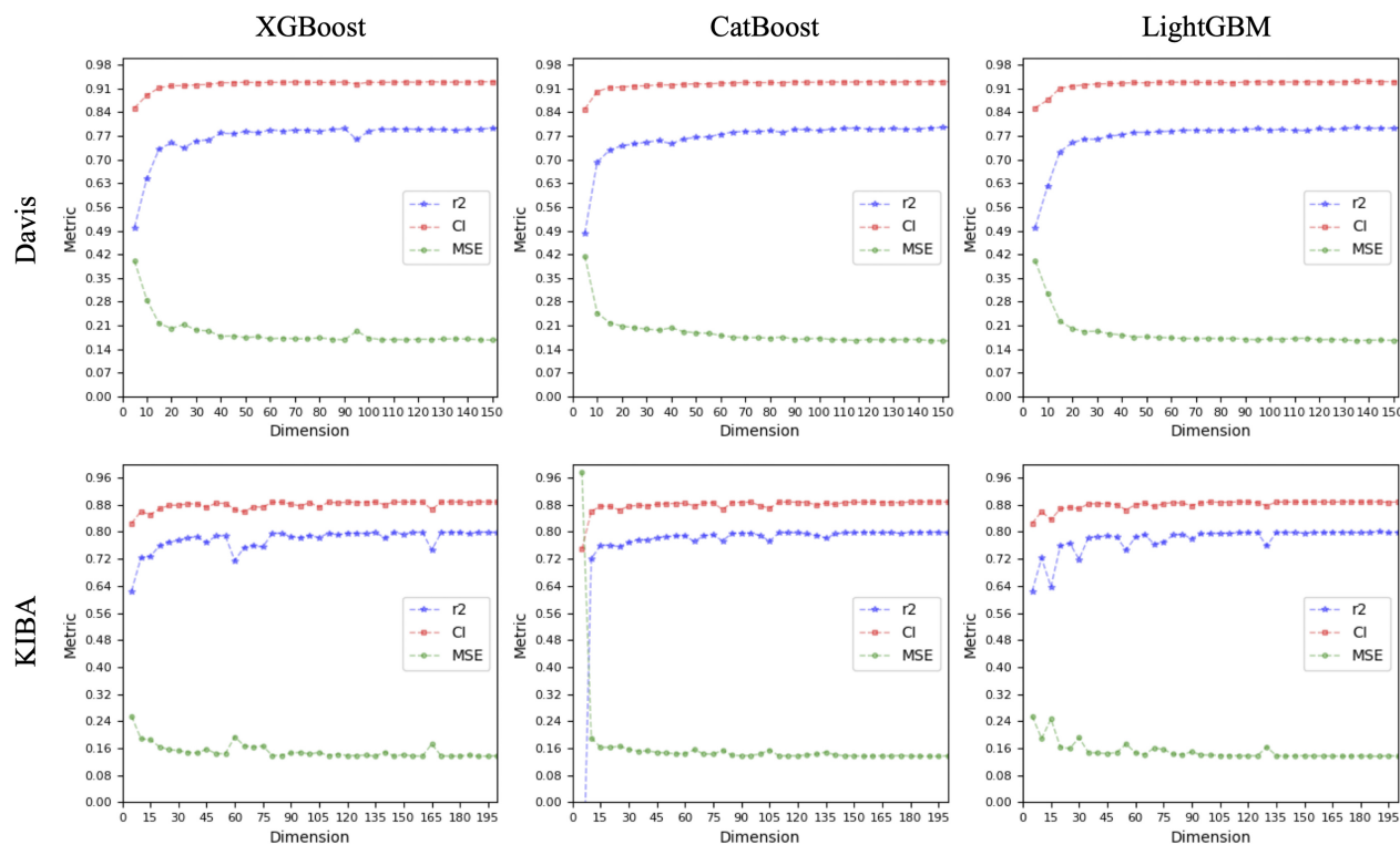
Figure 3. Performance of the model under each feature dimension on S2.
