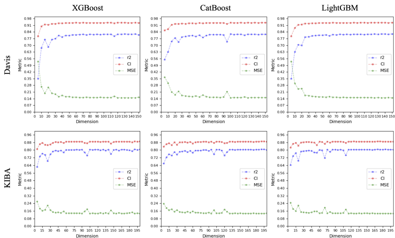
Figure 2. Performance of the model under each feature dimension on S1.
