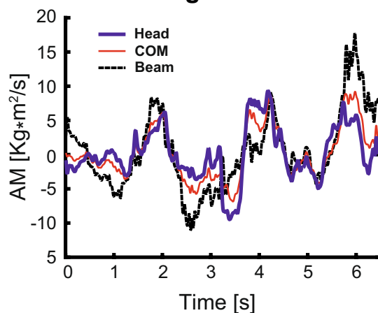
Figure 3. Temporal evolutions of the whole-body angular momentum during the first trial illustrated in Figure 2. The 3 lines refer to the axis through the head, the center-of-mass of the whole body, and the beam.
