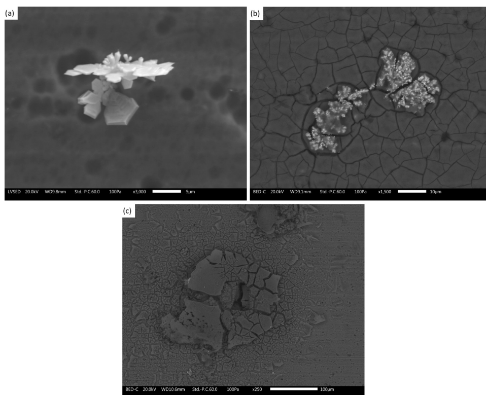
Figure 8. SEM micrographs of the surface of sample B after 1 day (a), 3 days (b), and 7 days (c) of the Kesternich test, respectively.
