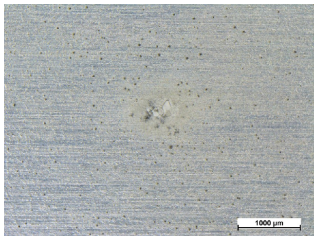
Figure 7. Optical micrograph of sample B with macro- and microdefects.
