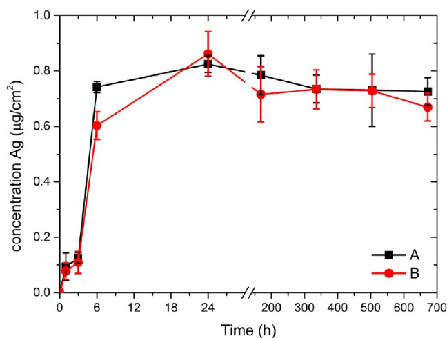
Figure 9. Ag ions release in synthetic sweat over time.
