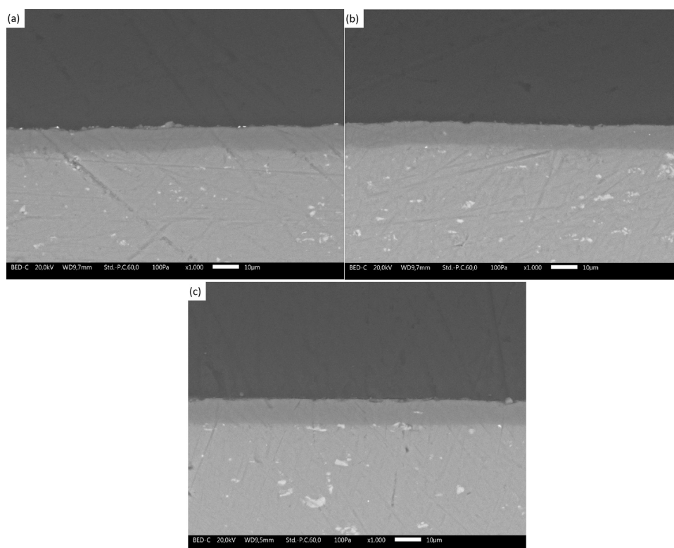
Figure 1. SEM micrographs of the cross section of sample X (a), sample A (b), and sample B (c), respectively.
