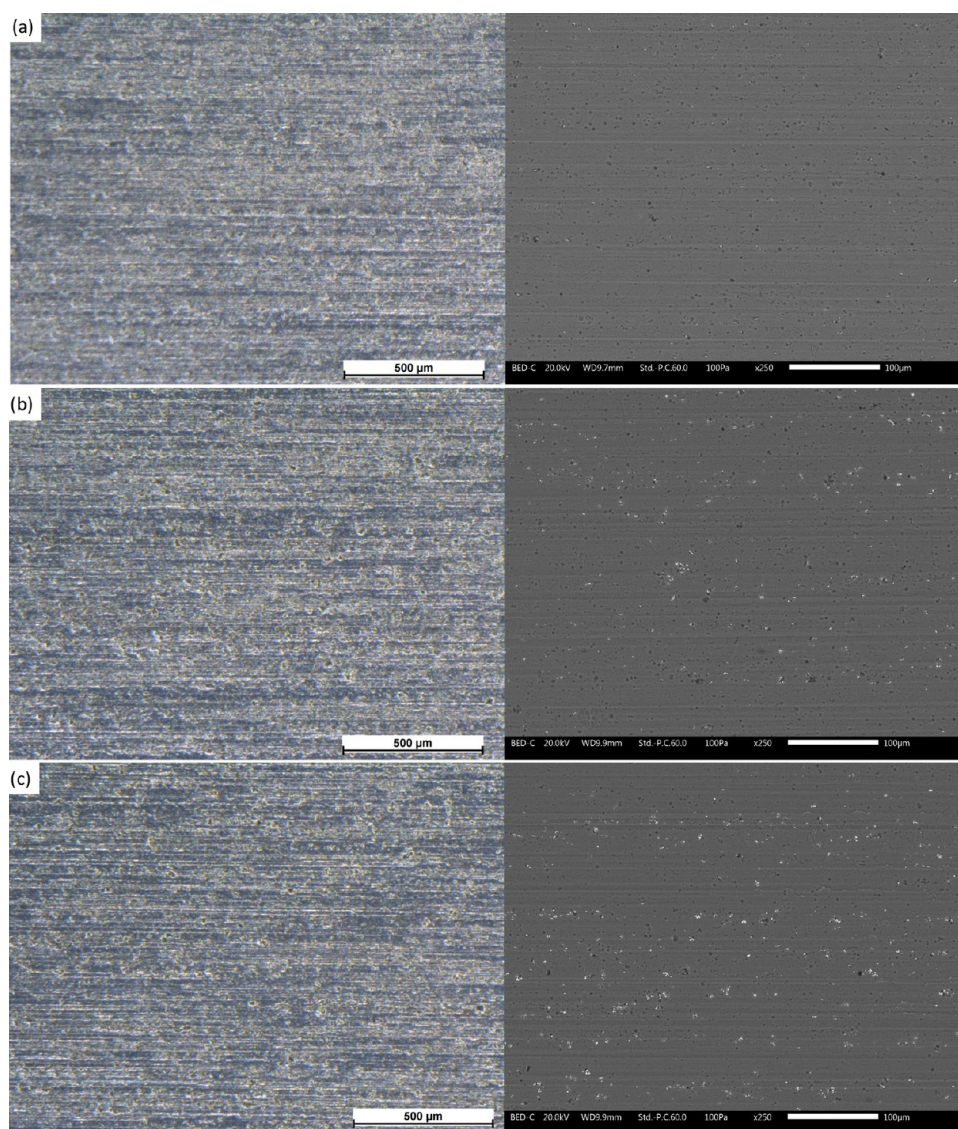
Figure 5. Micrographs of the surface of sample X (a), sample A (b), and sample B (c), respectively, after 7 days of exposure to UV-B radiation. The images on the left were collected by the optical microscope, while the corresponding ones on the right were acquired by the SEM.
