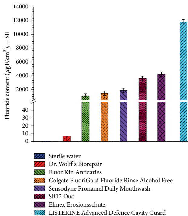
FIGURE 2: Results of the mean enamel fluoride uptake study ( n = 12 specimens).
