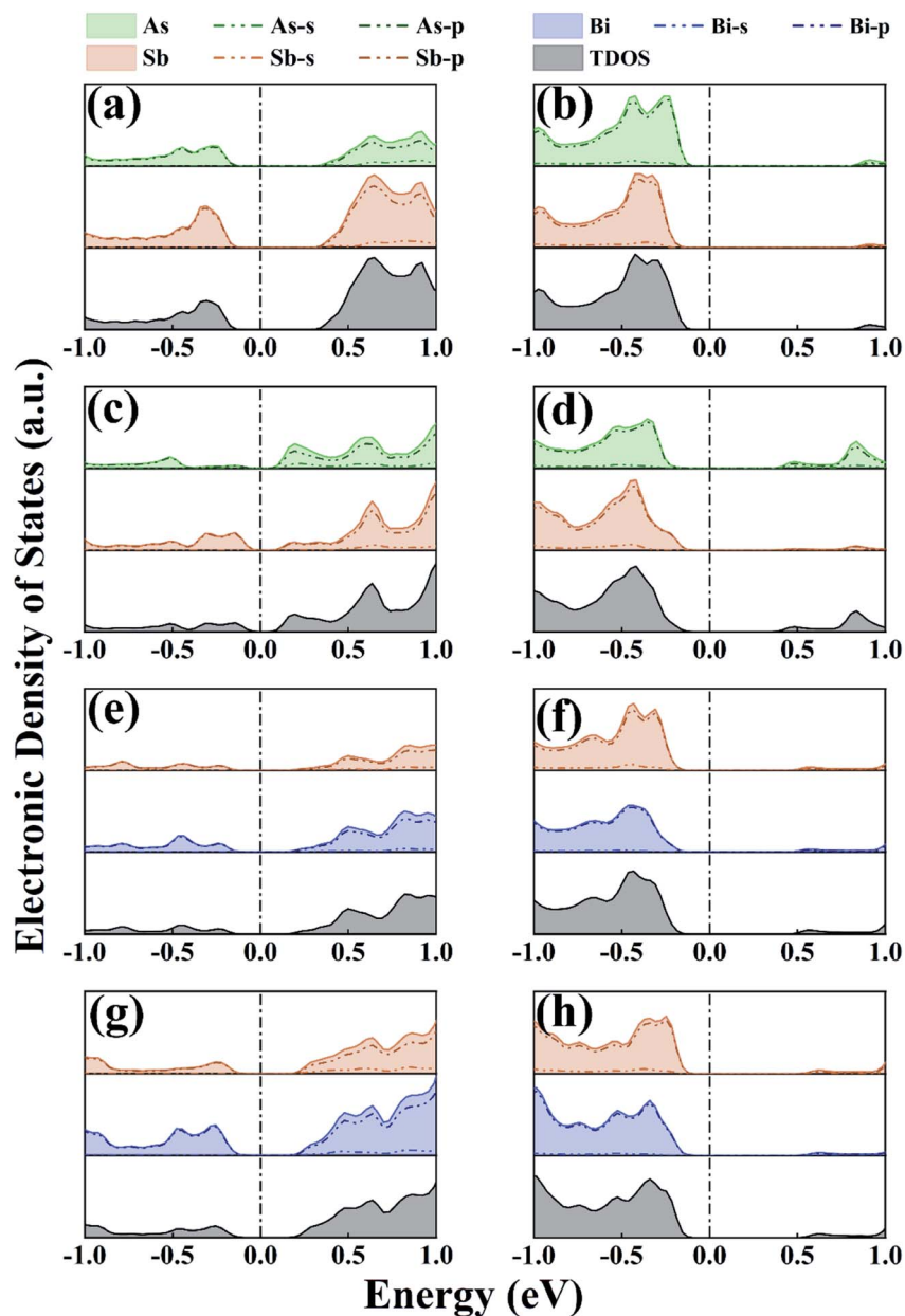
Fig. 4 PDOS for (a) armchair (AC) As/Sb lateral heterostructure (LHS) at -4\% strain, (b) AC As/Sb LHS at 4\% strain, (c) zigzag (ZZ) As/Sb LHS at -4\% strain, (d) ZZ As/Sb LHS at 4\% strain, (e) AC Sb/Bi LHS at -4\% strain, (f) AC Sb/Bi LHS at 4\% strain, (g) ZZ Sb/Bi LHS at -4\% strain, (h) ZZ Sb/Bi LHS at 4\% strain.
