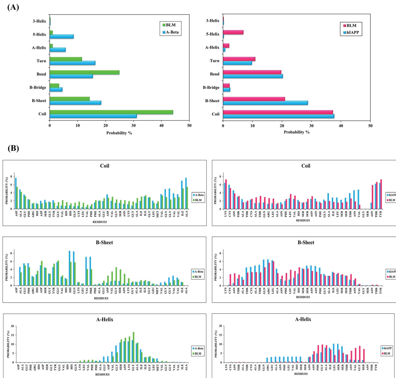
Fig. 6 (A) Probability% of secondary structures formation for A \beta and hIAPP in presence and absence of BLM. (B) Detailed residue specific probability% of secondary structures [coil (top), \beta -sheet (middle), and \alpha -helix (bottom)] for A \beta and hIAPP in presence and absence of BLM.
