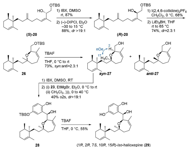
Scheme 5. Synthesis of iso -halioxepine 29 (o2s = over two steps).
