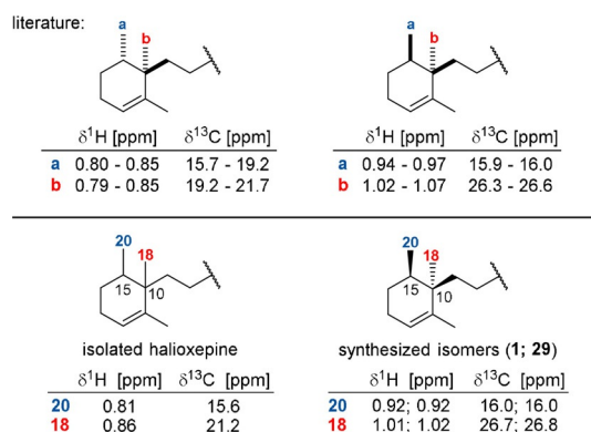
Figure 2. Comparison of 1 H- and 13 C-NMR shifts for cyclohexene-parts similar to those in halioxepine.
