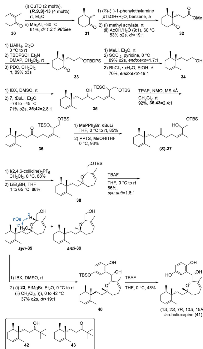
Scheme 6. Synthesis of altered western fragment 34 , coupling with eastern fragment 7 and synthesis of iso -halioxepine 41 (o2s = over two steps, o3s = over three steps).
