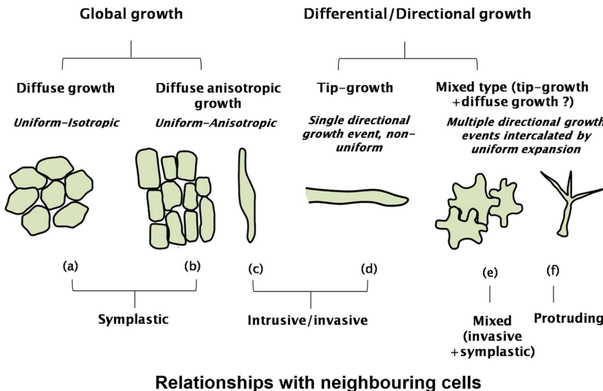
Figure 3. Cartoon depicting the two main plant cell growth events: global and differential/directional growth. Details concerning the cell types (a) fruit parenchyma cells; (b) shoot/root epidermal cells; (c) bast fibre; (d) pollen tube; (e) leaf pavement cells; (f) trichome and the relationship with the neighbouring cells are added to show the different expansion modalities displayed by plant cells. The question mark indicating the mixed-type growth refers to a hypothetical mechanism involving both tip- and diffuse growth.
