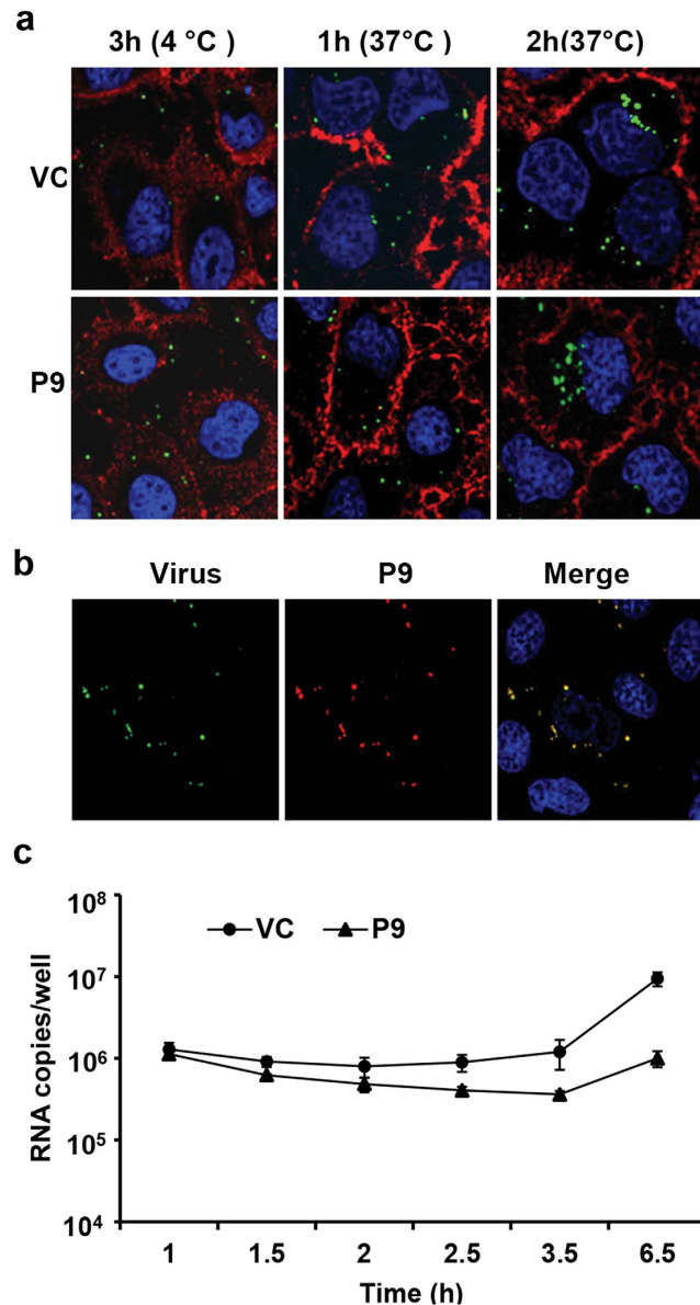
Figure 5. P9 did not inhibit virus-receptor binding or endocytosis but blocked viral RNA release. (a) P9 did not inhibit virus-receptor binding or endocytosis. DiO dye labeled virus pretreated with P9 or PB (VC) bound to the cell surface at 4 °C (left side) and entered the cells after incubation at 37 °C for 1 h or 2 h. The cell membrane was stained by Alexa-594 dye and representative images were taken by confocal microscope (original magnification 400×). (b) P9 was delivered into the cells by binding to the virus. Colocalization (orange) of virus (green) and P9 (red) was shown after incubation at 37 °C for 2 h. (c) P9 blocked the viral RNA replication. Viral RNA copies were detected in the cells infected with the virus pretreated with P9 or PB (VC) at the indicated time points. The results are presented as means ± SD of three independent experiments.
