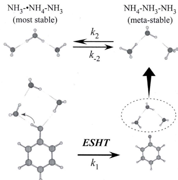
Fig. 8 ESHT reaction scheme for the PhOH-(NH 3 ) 3 cluster. The initial cluster (lower left) reacts at a rate k_1 to give the PhO \cdot ...NH 4 (NH 3 ) 2 product (lower right). The \cdot\text{NH}_4(\text{NH}_3)_2 dissociates from PhO \cdot (upper right) and then isomerizes to NH 3 \cdot -NH 4 NH 3 , the most stable isomer (upper left) at a rate k_2 . Reproduced from ref. 43 with the permission of AIP Publishing, copyright 2007.
