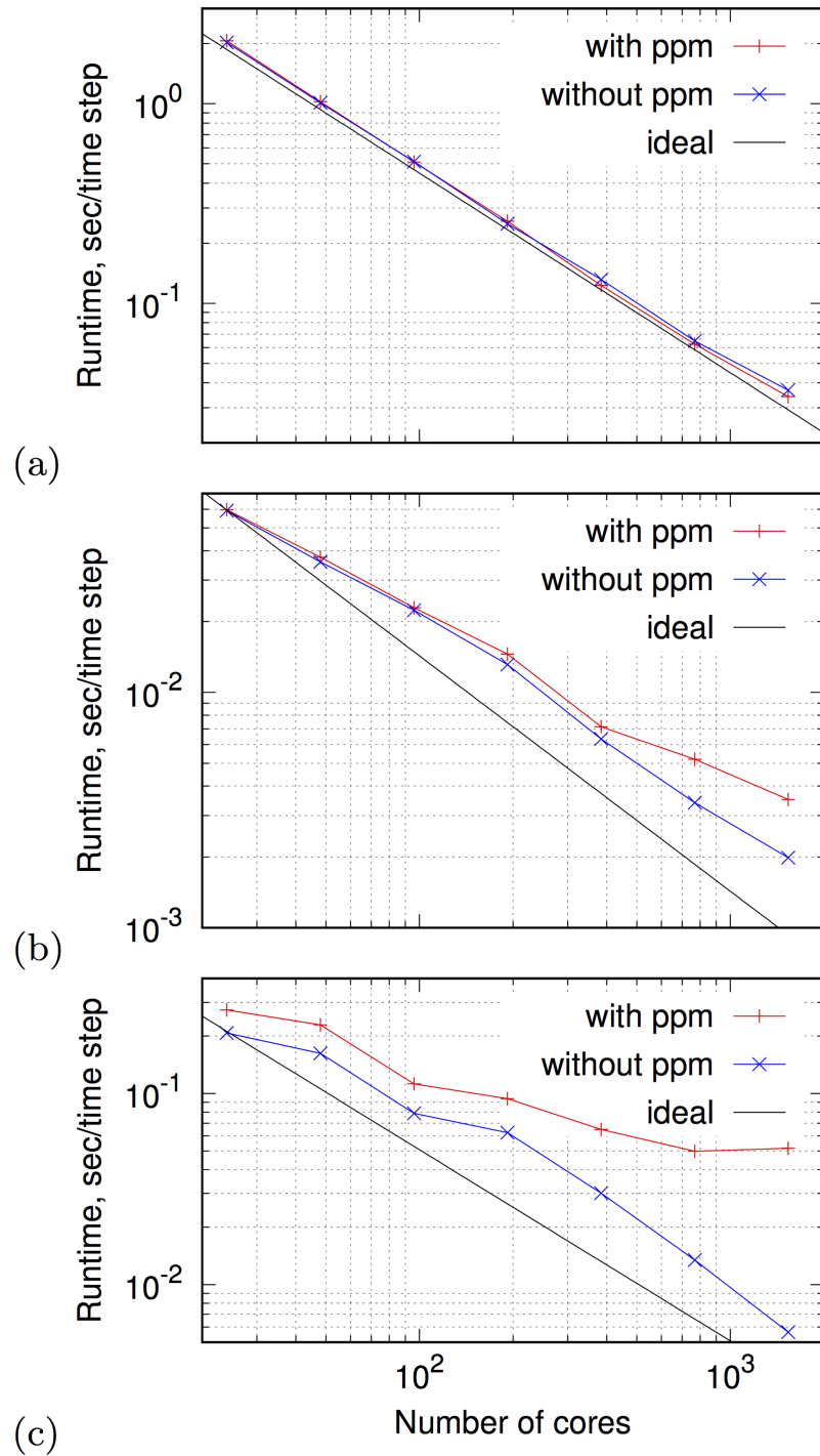
Fig 6. Log-log plots: The wall clock time per one time step in the simulation job, vs the number of cores. (a) Full box; (b) Rabbit ventricle geometry, (c) Human atrium geometry. In all plots, “with ppm” stands for performance including file output via ppmout device, “without ppm” stands for pure computations, and “ideal” is the perfect-scaling extrapolation of the performance achieved on the smallest number of cores.
