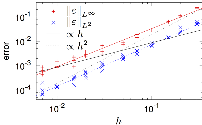
Fig 3. Numerical convergence of the solution of the problem Eqs (21)–(25). Slope lines are with slopes 1, 2 and best fits with slopes 1.564 for L ∞ , and 1.719 for L 2 .
