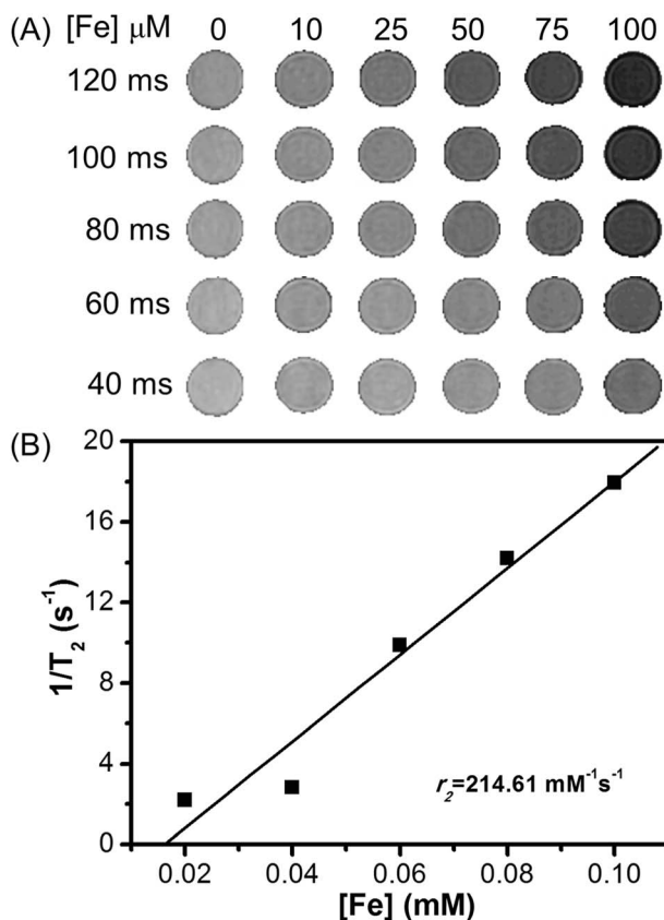
Fig. 5 Magnetic resonance imaging properties of \text{Fe}_3\text{O}_4/\text{HBC}@F127 nanocomposites: (A) T_2 -weighted MR images of \text{Fe}_3\text{O}_4/\text{HBC}@F127 nanocomposites in PBS solution at 3.0 T MRI system at various iron concentrations for different values of echo time (TE, TR = 3000 ms). (B) T_2 relaxivity plot of aqueous suspension of \text{Fe}_3\text{O}_4/\text{HBC}@F127 nanoparticles vs. iron concentration (data as values obtained from curve fitting).
