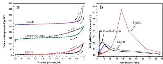
Fig. 4 \text{N}_2 adsorption–desorption isotherms and corresponding pore size distribution curves at 77\text{ K} of the dealloyed \text{Al}_{90}\text{Co}_{10} , \text{Al}_{90}\text{Sm}_{10} and \text{Al}_{90}\text{Co}_{9.5}\text{Sm}_{0.5} ribbons calcined at 300\text{ }^{\circ}\text{C} .
