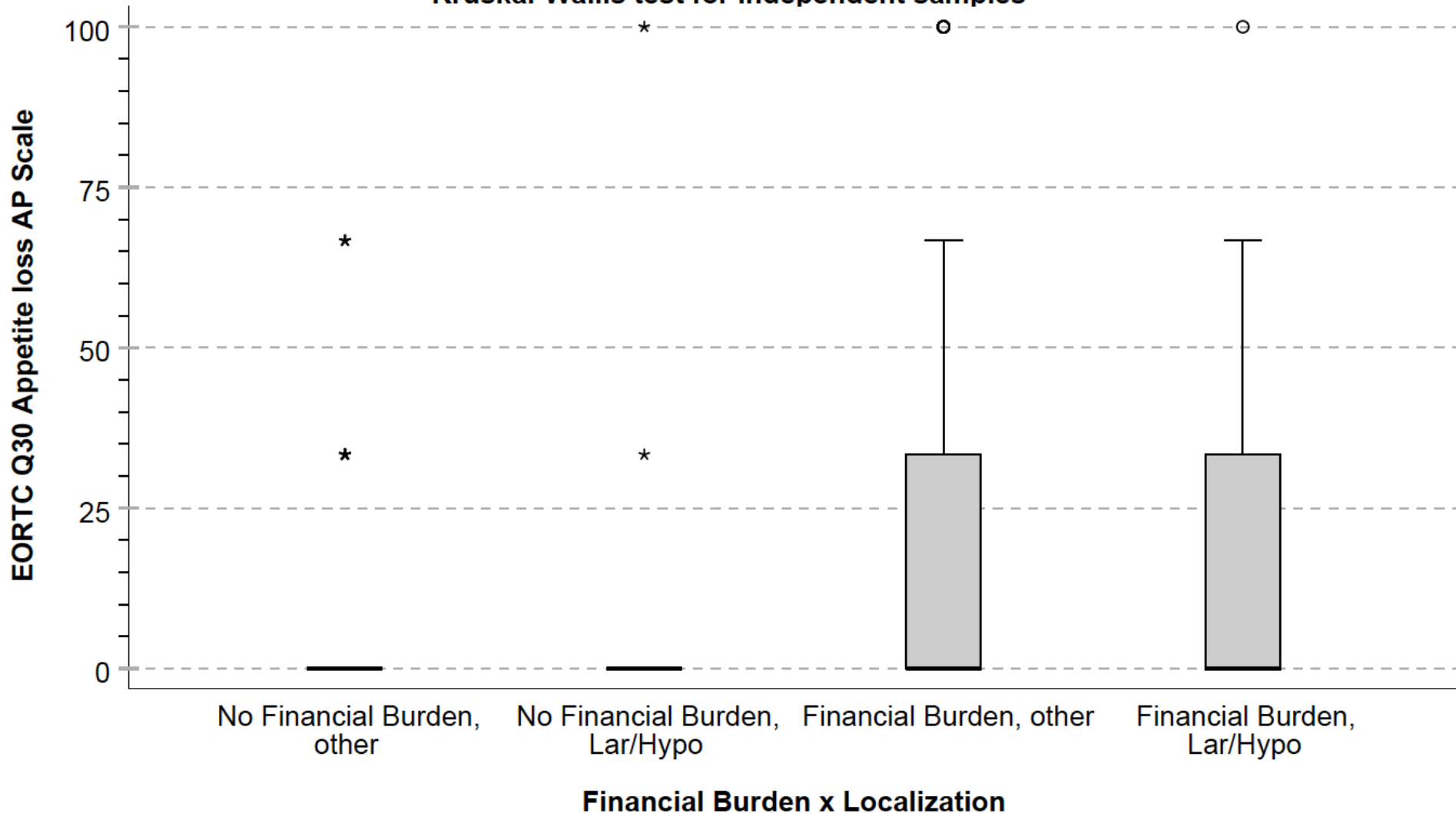
Kruskal-Wallis test for independent samples
