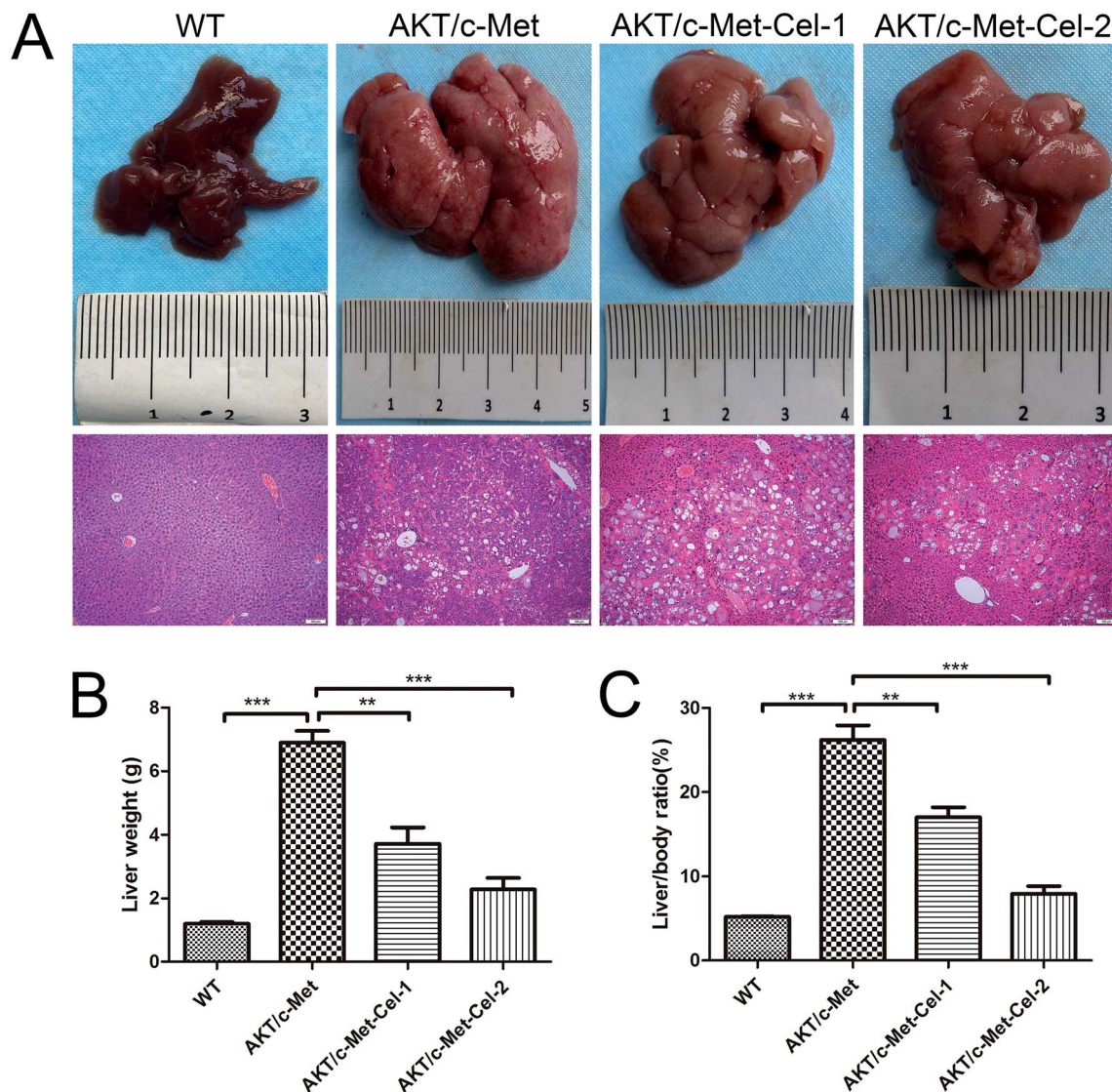
Fig. 1 Celastrol effectively inhibits tumor growth in AKT/c-Met HCC mice. (A) Macroscopic appearance and H&E staining (scale bar: 100 \mu\text{m} ) of AKT/c-Met mouse livers with celastrol treatment (1 or 2 \text{mg kg}^{-1} ) for 3 weeks. (B) The liver weight and liver/body ratio (C) of AKT/c-Met mice were both reduced by celastrol treatment. n = 5/\text{group} . **p < 0.01 ; ***p < 0.001 . AKT/c-Met-Cel-1 and AKT/c-Met-Cel-2 represent tumor burden groups with 1 or 2 \text{mg kg}^{-1} celastrol, respectively.
