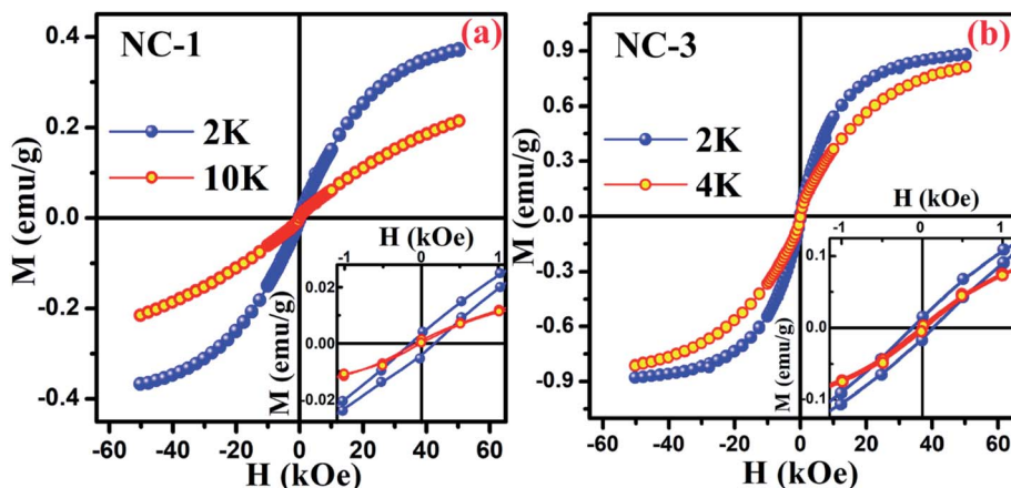
Fig. 14 Magnetic hysteresis loop for (a) NC-1 and (b) NC-3. Inset shows the enlarged view of the curves at low field region.
