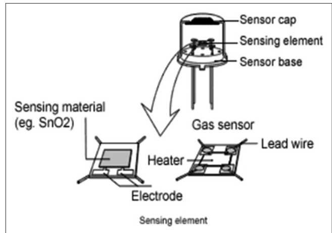
Figure 3: The gas sensor array instrumentation diagram
