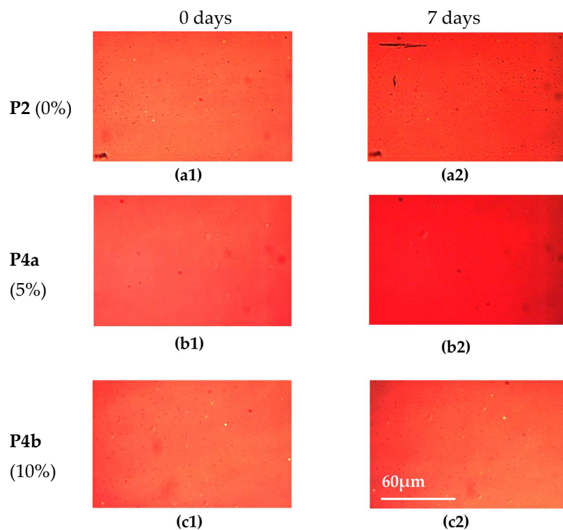
Figure 6. Optical microscope images (with 50× magnification) of the active layers of RC PSCs based on P2 (a), P4a (b) and P4b (c) after exposure to 85 °C for zero days (1) and seven days (2).
