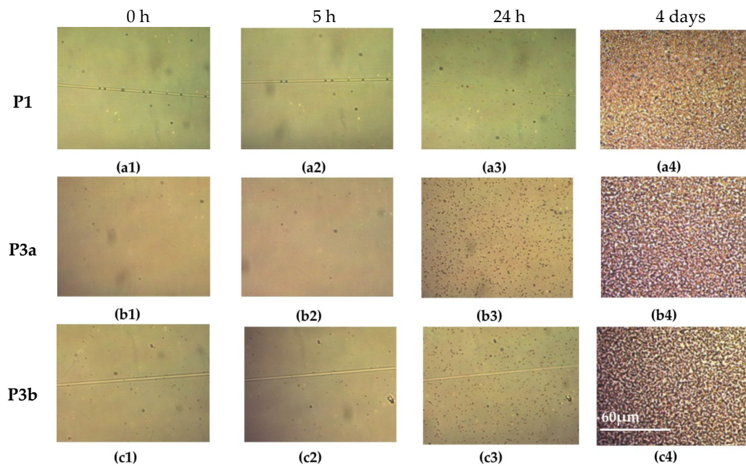
Figure 5. Optical microscope images (50× magnification) of the active layers of RC PSCs based on P1 (a), P3a (b) and P3b (c) after exposure to 85 °C for 0 h (1), 5 h (2), 24 h (3) and four days (4).
