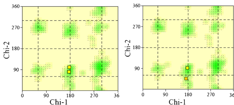
Figure 8 The \chi_1/\chi_2 plots are obtained from PROCHECK program. Each square represents one residue. The color coding of the squares is corresponding the range of yellow to red which is reflects the degree to which the orientation is favored; therefore, yellow indicate the residue is in a favored and red indicate the residue is an unfavored region. Two tryptophan of bovine serum albumin was indicated in both plots. The left plot indicate \chi_1/\chi_2 coordinate of tryptophans before MD (Left). The right plot indicates the \chi_1/\chi_2 coordinates of tryptophans after MD (Right). How it is shown, trp 134 remains constant while the \chi_1/\chi_2 coordinates of trp 212 is changed and located in unfavored region.
