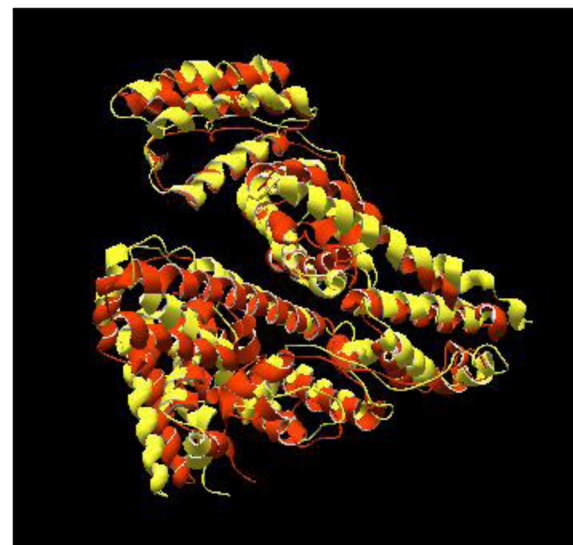
Figure 10 The superimposition between crystallographic structure of bovine serum albumin (PDB ID: 4F5S) (orange) and calculated 3D structure model (yellow), obtained with Swiss PDB viewer software.
