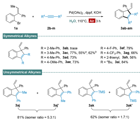
Scheme 3 Substrate scope of alkyne. Reaction conditions: 1a (0.30 mmol, 1.0 equiv.), 2b–m (1.2 equiv.), Pd(OAc) 2 (0.05 equiv.), dpfp (0.1 equiv.), KOH (0.60 mmol, 2.0 equiv.), H 2 O (1.5 mL), a C 12 H 25 SO 4 Na (1.0 equiv.) b 2 wt% solution of TPGS-750 M/H 2 O (1.5 mL).
