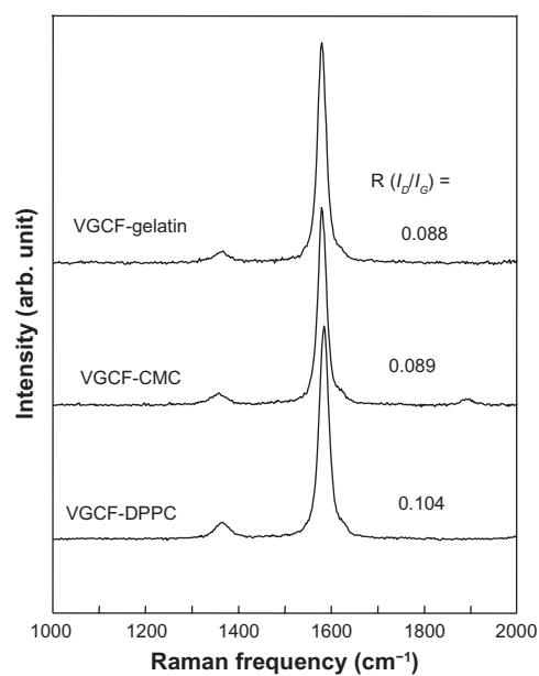
Figure S4 Raman spectroscopy of vapor grown carbon fiber (VGCF®) in different dispersants.
