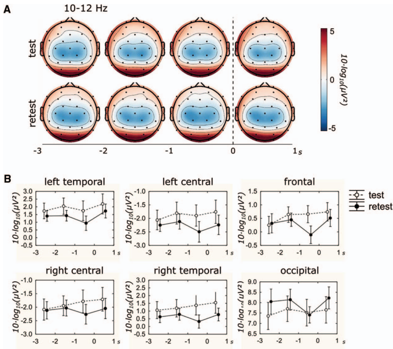
Figure 1. (A) Scalp maps representing alpha power [ 10 \cdot \log_{10}(\mu V^2) ] averaged across participants, as a function of session (test, retest), time (-3 to +1 s), and channel. (B) Alpha power [ 10 \cdot \log_{10}(\mu V^2) ] averaged across participants, as a function of session (test, retest) and time (-3 to +1 s) in the six regions. Error bars represent the standard error of the mean. See the online article for the color version of this figure.
