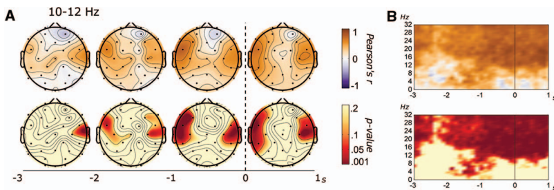
Figure 3. (A) Scalp maps representing Pearson's correlations conducted on the inter-session change scores between the number of holed putts and alpha power, as a function of time ( -3 to +1 s) and channel. (B) Time-frequency plots representing Pearson's correlations conducted on the inter-session change scores between the left temporal alpha power [ 10 \cdot \log_{10}(\mu V^2) ] and the number of holed putts, as a function of time ( -3 to +1 s) and frequency ( 0 to 32 Hz). See the online article for the color version of this figure.
