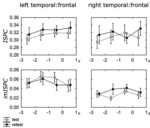
Figure 2. Left/right temporal:frontal alpha ISPC and imISPC averaged across participants as a function of session (test, retest) and time ( -3 to +1 s). Error bars represent the standard error of the mean.
