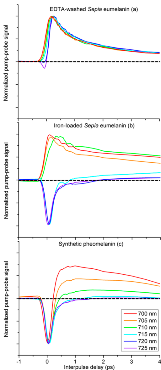
Figure 2. Pump–probe response of dry melanins. Probe wavelength is set at 815 nm. Pump wavelength is varied from 700 to 725 nm. Data are normalized to the largest peak and smoothed using a 5 point, second-degree polynomial Savitzky–Golay filter to facilitate comparison of response curves with variable SNR levels. 16
