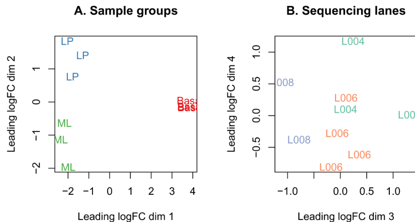
Figure 3. MDS plots of log-CPM values over dimensions 1 and 2 with samples coloured and labeled by sample groups (A) and over dimensions 3 and 4 with samples coloured and labeled by sequencing lane (B). Distances on the plot correspond to the leading fold-change, which is the average (root-mean-square) \log_2 -fold-change for the 500 genes most divergent between each pair of samples by default.
