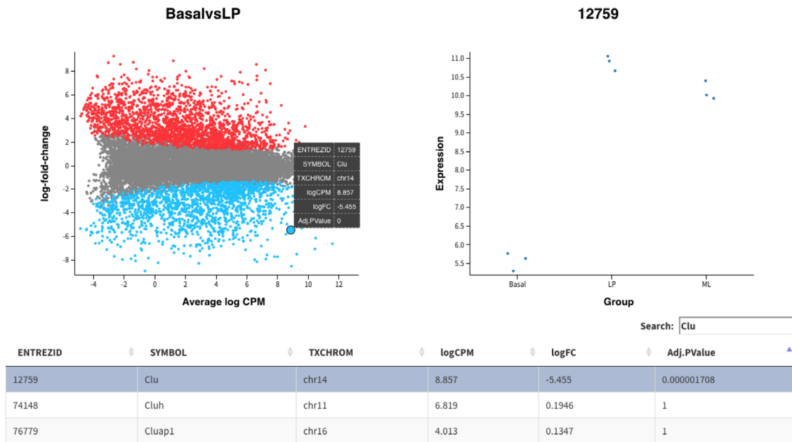
Figure 6. Interactive mean-difference plot generated using Glimma. Summary data (log-FCs versus log-CPM values) are shown in the left panel which is linked to the individual values per sample for a selected gene in the right panel. A table of results is also displayed below these figures, along with a search bar to allow users to look up a particular gene using the annotation information available, e.g. the Gene symbol identifier Clu .
