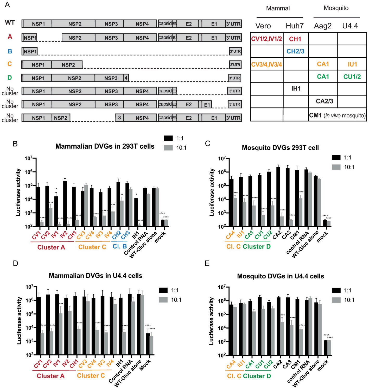
Fig 3. Defective viral genomes can interfere with chikungunya virus replication. (A) Schematic of the DVG candidates and the cell type and strain from which they were derived (C Carib, I IOL). (B-E) Measuring DVG activity in vitro . In vitro transcription of each DVG candidate (identified from mammalian cell passage (B,D) or mosquito cell passage (C,E)) or of a control RNA was co-transfected with CHIKV Carib-luciferase at 1:1 or 10:1 molar ratio in 293T cells (B,C) or U4.4 cells (D,E). After 48 hours, luciferase activity was measured. (Representative result of one experiment out of three independent experiments is shown, n = 3, *p<0,05, **p<0,01, ***p<0,001, ****p<0,0001, ns non significant compared to wild-type after Dunnett’s multiple comparisons on one-way ANOVA test).
