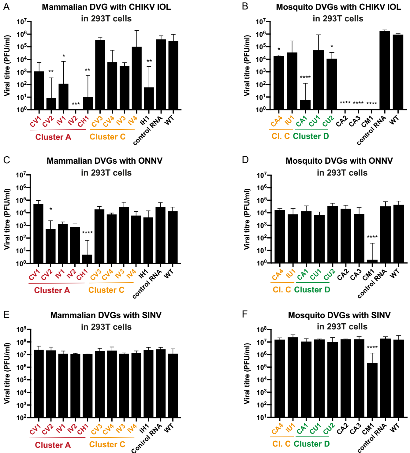
Fig 4. Defective viral genomes have broad-spectrum inhibiting activity in the alphavirus family. The DVGs identified in mammalian cell passage (A,C,E) or mosquito cell passage (B,D,F) were tested for inhibition of CHIKV IOL (A,B), O'nyong-nyong virus (ONNV) (C,D) and Sindbis virus (SINV) (E,F). In vitro transcribed DVG candidates were co-transfected with CHIKV IOL (A,B), ONNV (C,D) and SINV (E,F) at 10:1 molar ratio in 293T cells. After 48 hours, viral titer was measured. (Representative result of one experiment out of three, n = 3, *p<0,05, **p<0,01, ***p<0,001, ****p<0,0001, ns non-significant compared to wild-type after Dunnett's multiple comparisons on one-way ANOVA test).
