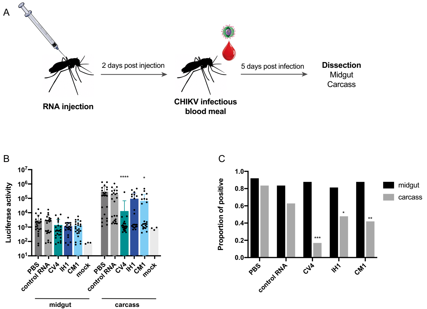
Fig 5. Defective viral genomes prevent viral dissemination of chikungunya virus in Aedes aegypti mosquitoes. (A) 150 ng of DVG candidate RNA (IH1, CV4 or CM1), a control RNA or PBS were injected into Aedes aegypti mosquitoes 2 days prior to being fed an infected blood meal containing 10 6 PFU/ml. After 5 days, mosquitoes were sacrificed, and midguts were separated from carcasses. (B) Luciferase activity of midgut or carcass of each mosquito was measured. (C) After virus titration, the proportions of positive midguts or carcasses (PFU ≥ 100 PFU/ml) were determined. (Representative result of one experiment out of two independent experiments is shown, n = 24, *p < 0,05, **p < 0,01, ***p < 0,001, ns non significant compared to PBS after one-way ANOVA with multiple comparison (B) or Chi square test, multiple comparison with Holm correction (C)).
