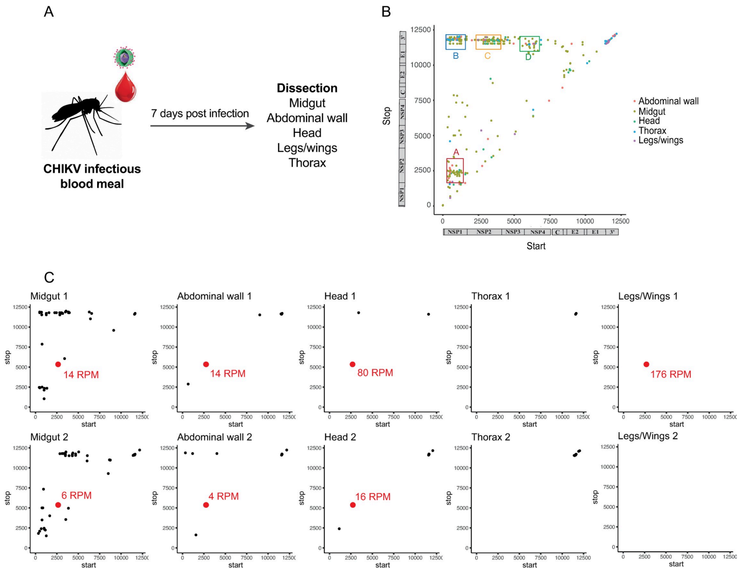
Fig 2. Generation of chikungunya DVGs in mosquitoes in vivo . (A) Aedes aegypti mosquitoes were fed a blood meal infected with 10^6 PFU/ml of CHIKV Carib. After 7 days, ten mosquitoes were sacrificed and midgut, abdominal wall (body), thorax, head and legs/wings were dissected. After verification of infection by titration, viral RNA was extracted and deep-sequenced. (B) Analysis of the deletions generated by CHIKV Carib in nine infected mosquitoes pooled together. Start (x axis) and stop (y axis) positions of the breakpoint of DVGs generated are plotted for each organs. (C) Start (x axis) and stop (y axis) positions of the breakpoint of DVGs generated in the different organs of 2 individual mosquitoes. The red dots represent the deletion starting at 2695 and ending at 5358, this DVG is called CM1. The number next to it is the number of read per million reads (RPM).
