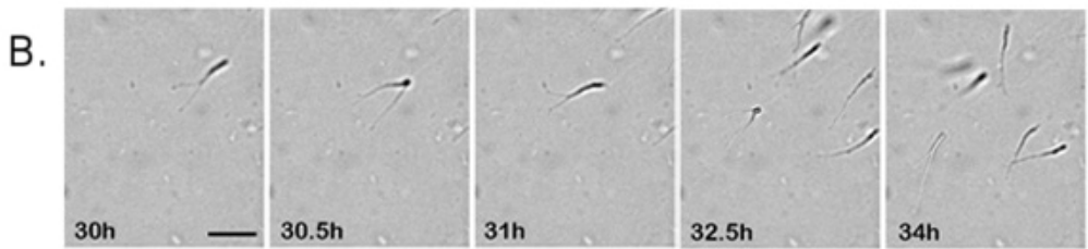
Figure 4. A) A series of images from selected timepoints showing a growing cloud of cells migrating out of an explant. An example cell, indicated by an arrow, is tracked through time as indicated below (scale bar 200µm). This explant was visualized with live imaging for 38 h. Shown here
