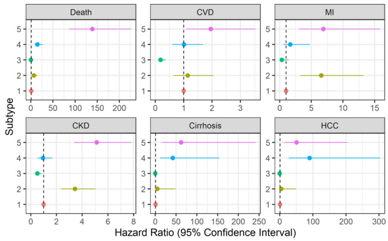
Fig. 2. Univariate hazard ratios for outcomes of interest, by 5 subtypes
