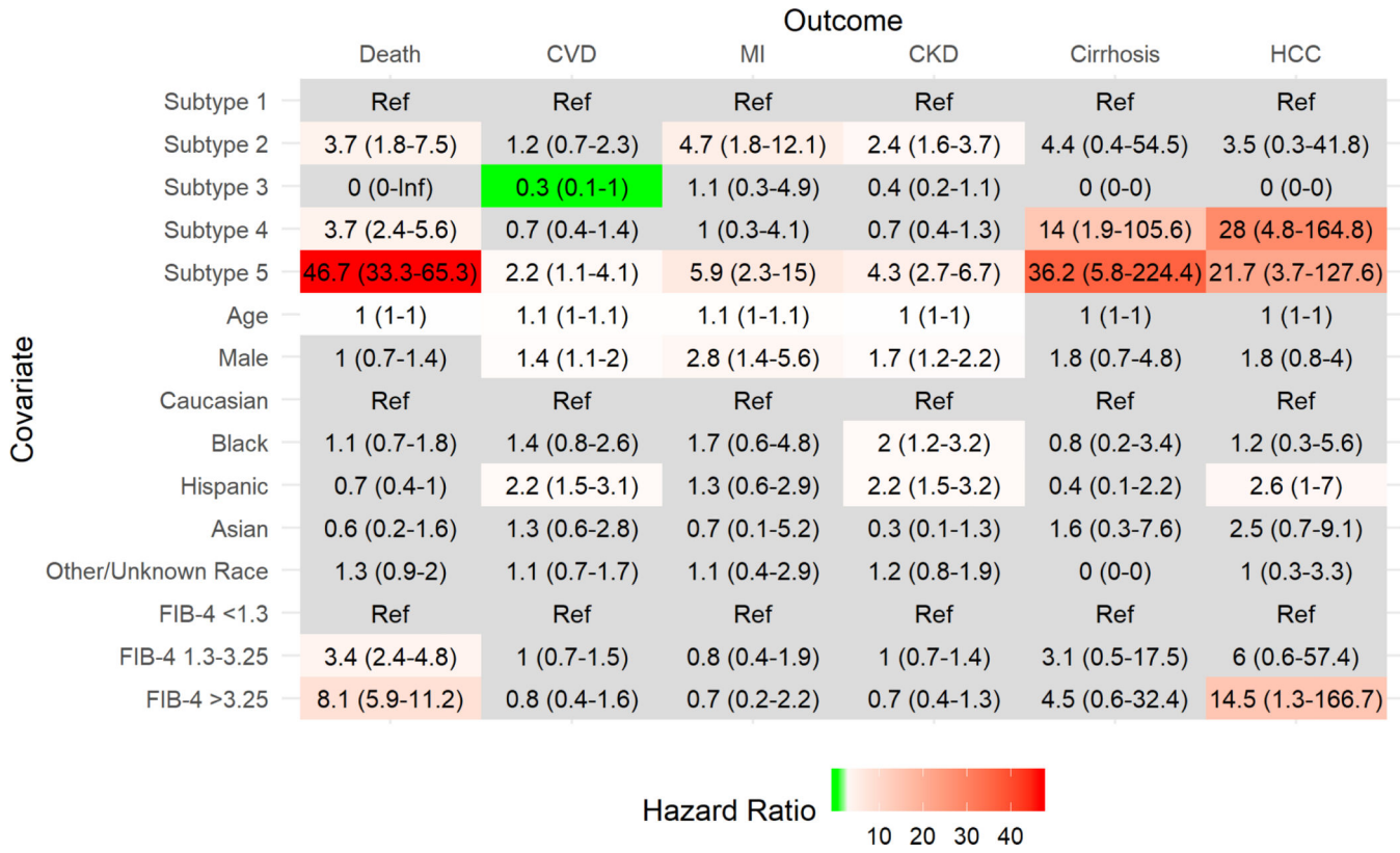
Fig. 3. Multivariate analyses for outcomes of interest. Darker shades of red correlate with increased risk of the outcome, while darker shades of green indicate reduced risk of the outcome. Only hazard ratios with p < 0.05 are color coded. Non-significant findings are in grey.
