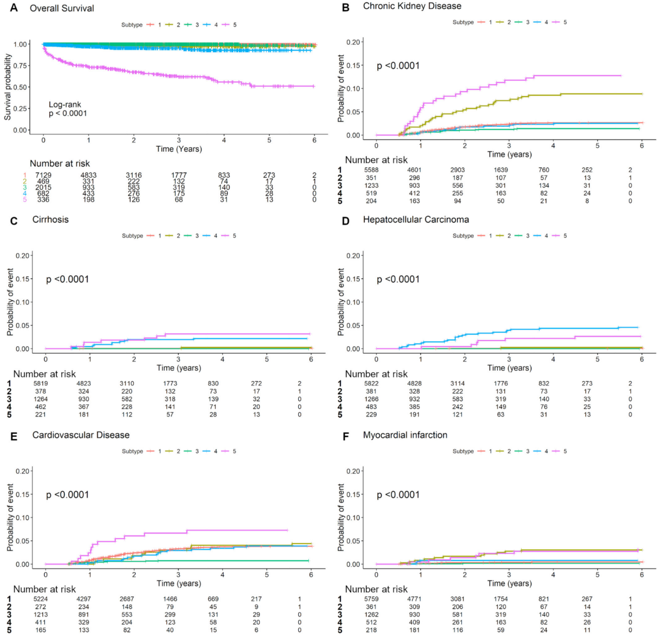
Fig. 1. Survival and hazard curves for outcomes of interest, 5 by subtypes. (A) Overall survival, (B) Chronic kidney disease, (C) Cirrhosis, (D) Hepatocellular carcinoma, (E) Cardiovascular disease, (F) Myocardial infarction.
