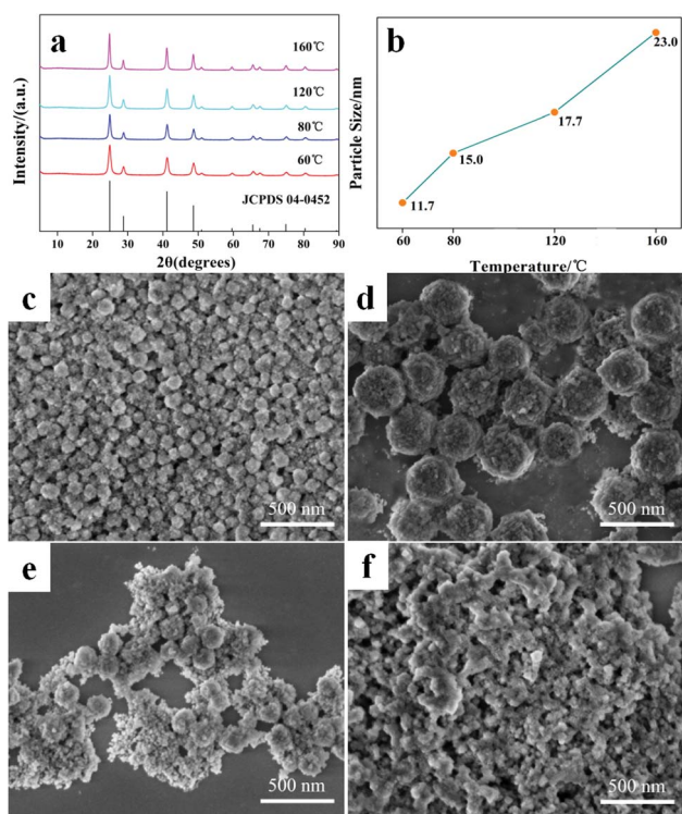
Fig. 5 (a) XRD patterns of BaF 2 samples prepared at different hydrothermal temperatures; (b) the particle size calculated by the Scherrer formula; SEM images of BaF 2 samples prepared at different hydrothermal temperatures (c) 60 °C, (d) 80 °C, (e) 120 °C, (f) 160 °C.
