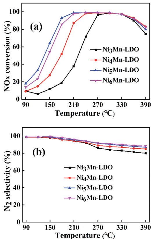
Fig. 5 (a) \text{NO}_x conversion and (b) \text{N}_2 selectivity of \text{Ni}_x\text{Mn-LDO} ( x = 3, 4, 5, 6 ) catalysts. Reaction conditions: [\text{NO}] = [\text{NH}_3] = 600\text{ ppm} , [\text{O}_2] = 5\text{ vol\%} , \text{N}_2 as balance gas, GHSV = 45\,000\text{ h}^{-1} .
