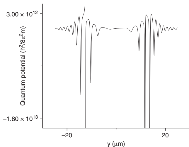
Fig. 4 The Quantum Potential. The potential, -\hbar^2\nabla^2A/2mA , is calculated from the wavepacket Ae^{i\phi} that is propagated 1% of the distance from the magnetic flux line to the detection plane. The wavefunction is obtained from the path integral calculation. The left-right asymmetry is caused by the phase shift induced by the magnetic flux line and illustrates why the word “force” can be used in the present context
