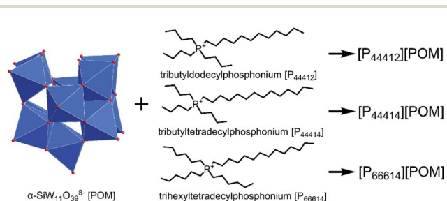
Fig. 1 Schematic illustration of the [P 44412 ][POM], [P 44414 ][POM], and [P 66614 ][POM].
