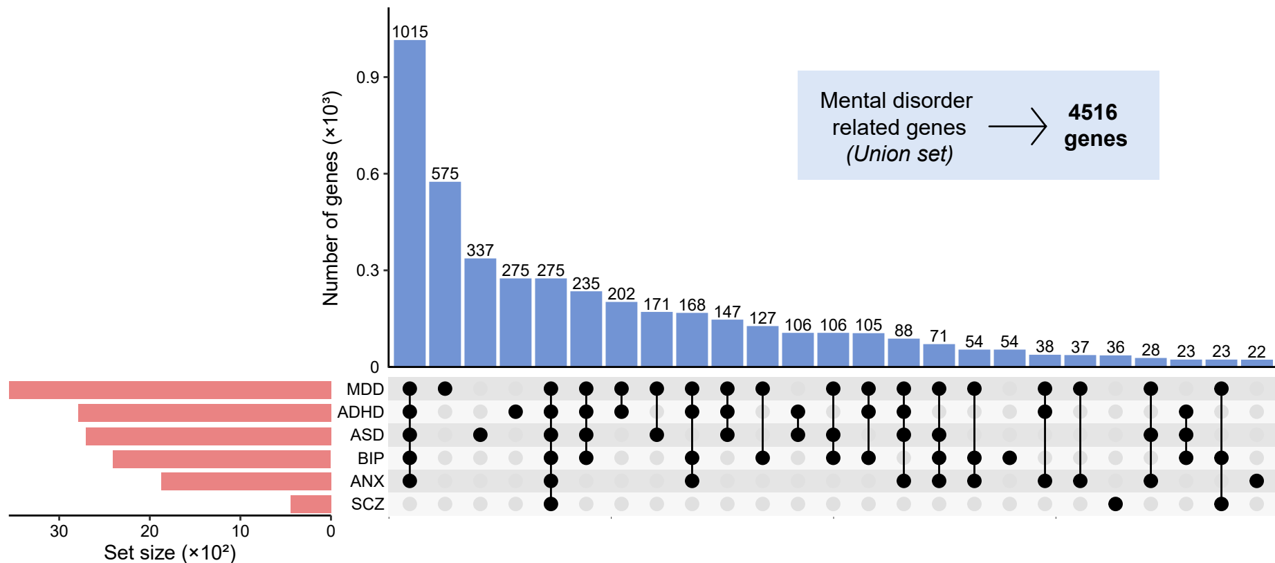
Fig S1. Candidate mental disorder-related genes. The UpSet plot exhibited the intersection of genes of six mental disorders.
