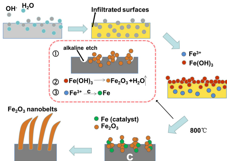
Figure 4. Schematic illustrating in-situ catalytic growth of \text{Fe}_2\text{O}_3 nanobelts during high-temperature carbonization of an alkali activated cotton leading to \text{Fe}_2\text{O}_3 /NPCTT.
