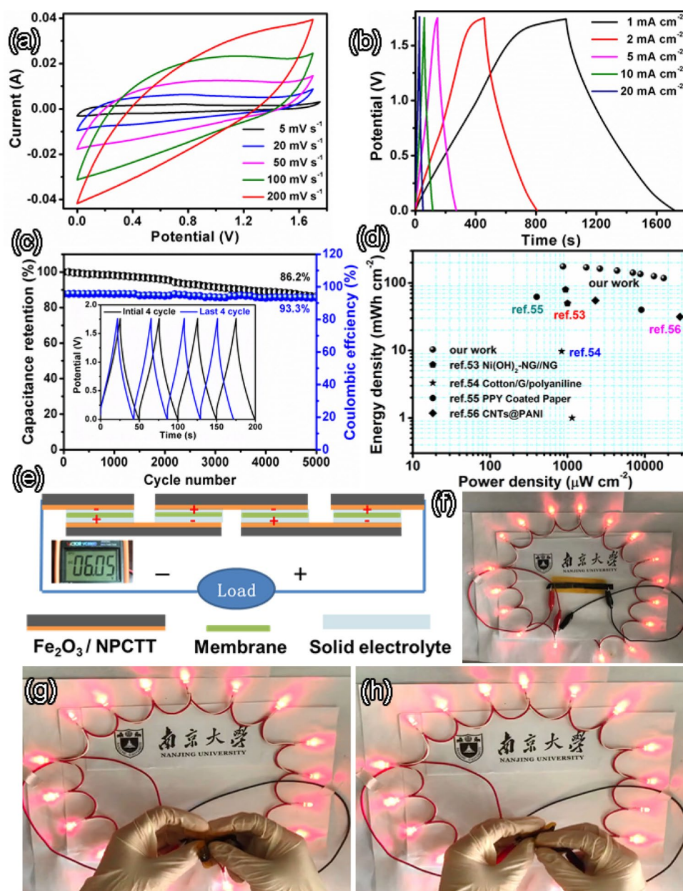
Figure 7. (a) CV curves at various scan rates, (b) GCD curves at different current densities of an solid-state symmetric supercapacitor with \text{Fe}_2\text{O}_3/\text{NPCTT} electrode, and (c) Cycling performance and Coulombic efficiency of the supercapacitor (measured at a high current density of 20 \text{ mA cm}^{-2} ) with an inset showing the initial and last four cycles; (d) Ragone plots of our device with comparison to previous reports. (e) Schematic illustrations of assembled structure of a tandem by connecting four SCs in series; (f) Digital photos showing 18 LEDs powered by the tandem, and (g) the tandem being fully folded (bending angle 180^\circ ) and (h) being largely twisted.
