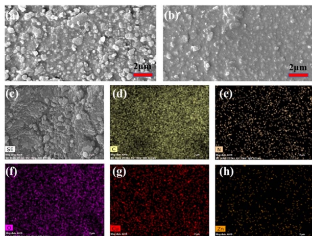
Fig. 6 (a) FE-SEM image of compound 2 before testing; (b) SEM image of compound 2 after testing; (c–h) EDX-mapping analysis of each element in compound 2.
