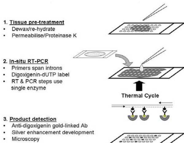
Figure 2 Flow chart describing the application of in situ RT-PCR to tissue microarrays. Step 1: Slide preparation. Sections were deparaffinated by xylene washes, and cellular material permeabilised by limited proteinase K digestion; Step 2: amplification of reverse-transcribed cDNA using intron-spanning PCR primers (horizontal arrows) added in a single mix of reverse transcriptase, rTth polymerase and deoxyribonucleotides spiked with digoxigenin-labelled dUTP (black ovals); Step 3: visualisation of PCR products by binding to digoxigenin-specific gold-labelled antibodies (yellow dots), followed by silver nucleation around the bound gold particles (grey crescents).
