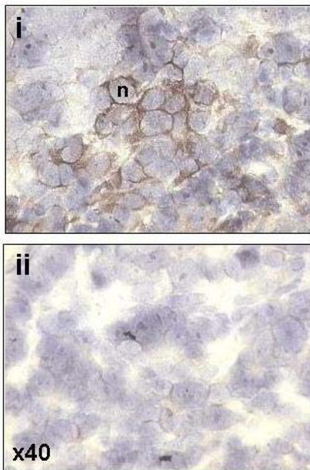
Figure 3 In situ RT-PCR analysis of tissue microarrays. Slides containing up to 250 sections of 1 mm diameter, taken from prostate cancer biopsies, were subjected to in situ RT-PCR as described in Methods, using either spondin-2-specific oligonucleotide primers (i) or control 'scrambled' primers (ii). PCR products were labelled by Immunogold with silver enhancement; after hematoxylin staining to highlight cell nuclei (n), sections were visualised by light microscopy at 40 \times magnification.
