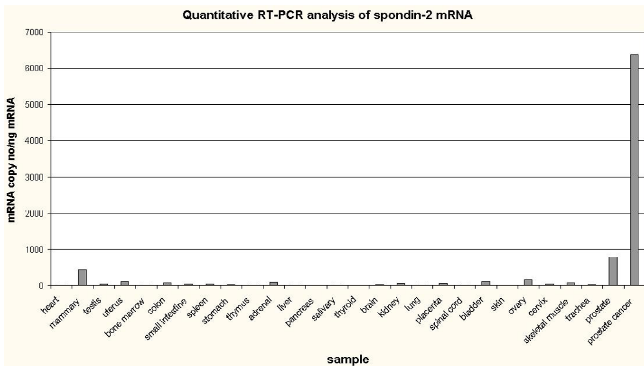
Figure 1 Quantitative RT-PCR analysis of human primary normal and cancer tissues. Amplification of reverse-transcribed mRNA was carried out on pools of normal human tissue as indicated and on a pool of prostate cancer samples, as described in Methods, and measured by SYBR-green staining and fluorescence quantification. Results were calculated relative to a set of standards and expressed here as copy number of original transcripts per ng of mRNA.
