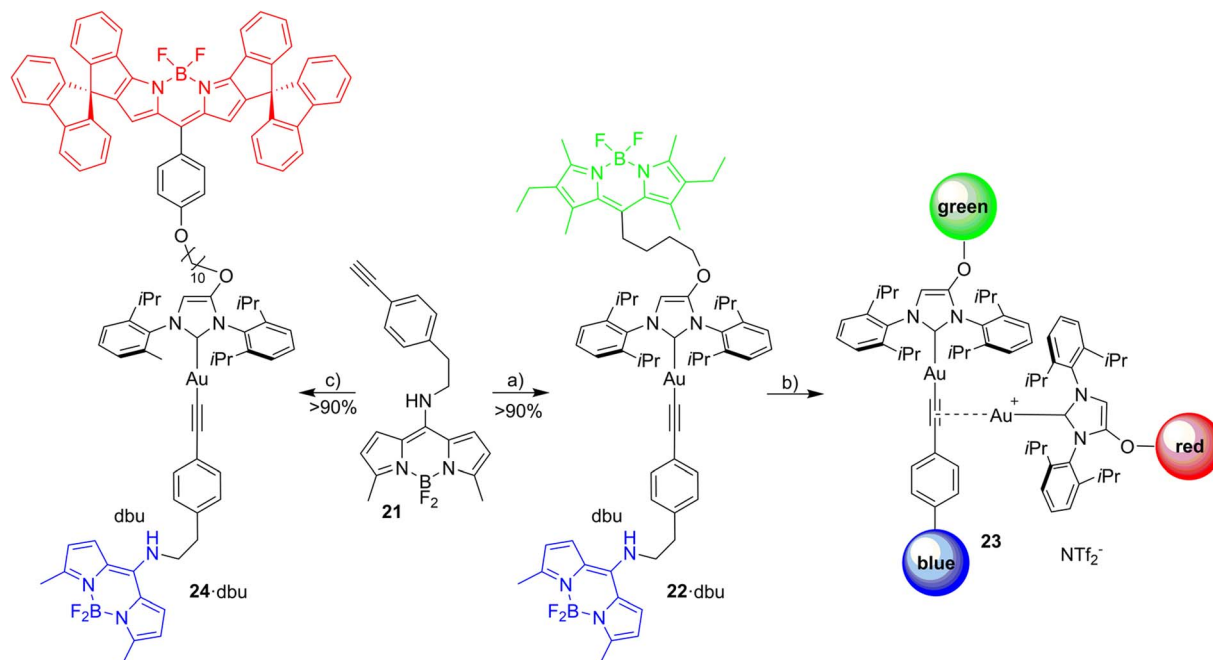
Scheme 8 Synthesis of the blue-green dyad and the blue-green-red triad. Reagents and conditions: (a) [\text{AuCl}(\text{NHC\_green})] , dbu, \text{CH}_2\text{Cl}_2 ; (b) [\text{Au}(\text{NTf}_2)(\text{NHC\_red})] 14 in 1,2-dichloroethane; (c) [\text{AuCl}(\text{NHC\_red})] , dbu, \text{CH}_2\text{Cl}_2 .
