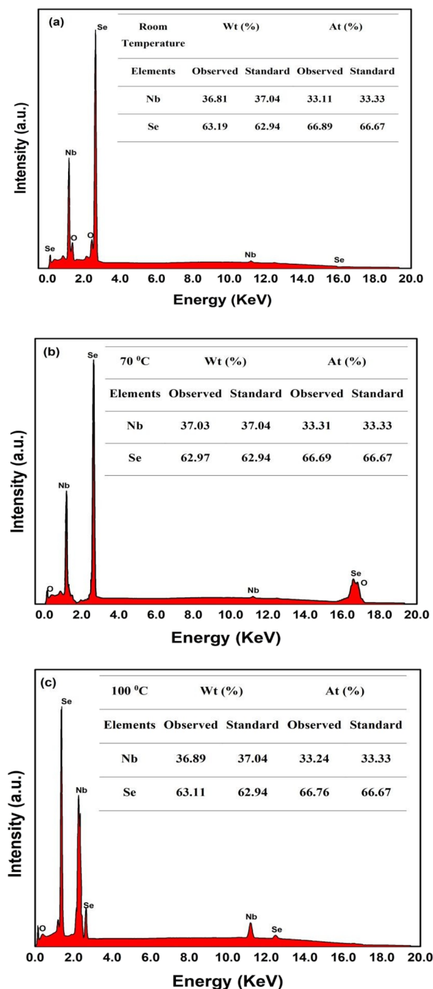
Fig. 1 The EDAX spectrum of NbSe 2 NPs synthesized at (a) R.T., (b) 70 °C, and (c) 100 °C.
