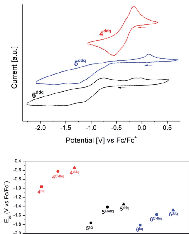
Fig. 3 Top: Stacked cyclic voltammograms of complexes 4 ddq (red), 5 ddq (blue), 6 ddq (black) in THF ( \nu = 50 \text{ mV s}^{-1} ; c(\text{analyte}) = 2 \text{ mM} ; c([\text{InPr}_4\text{N}][\text{B}(\text{C}_6\text{H}_3(\text{CF}_3)_2-3,5)_4]) = 0.1 \text{ M} ). Bottom: comparison of the second reduction potentials of complexes 4 (red), 5 (black), and 6 (blue) in THF vs. \text{Fc}/\text{Fc}^+ . Squares: complexes with bridging 1,4-hydroquinolates; circles: complexes with bridging tetrachloro-1,4-hydroquinolates; triangles: complexes with bridging 2,3-dichloro-5,6-dicyano-1,4-hydroquinolates.
