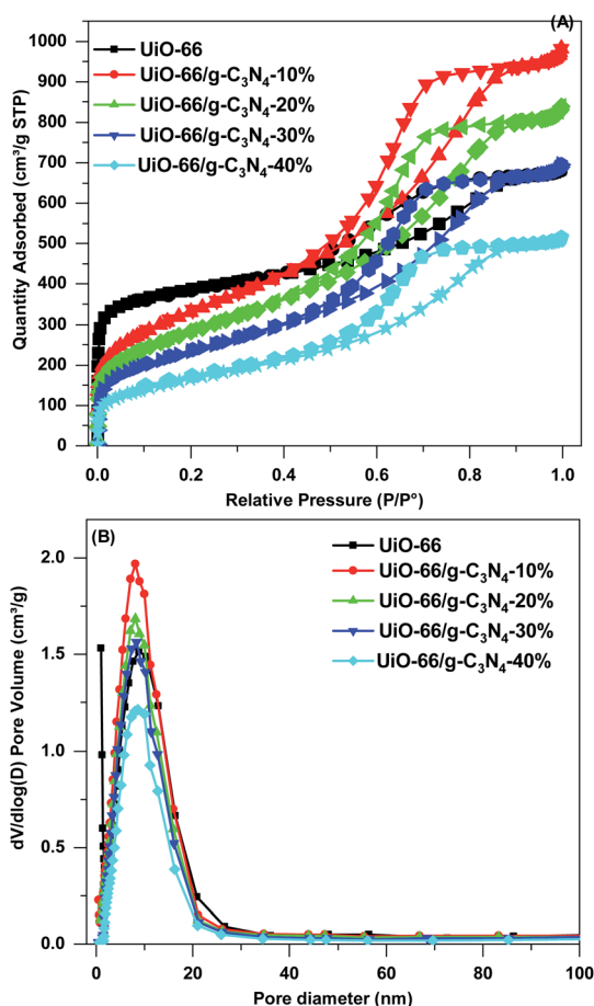
Fig. 4 (A) N_2 adsorption–desorption isotherms and (B) pore size distributions of UiO-66 and UiO-66/g- C_3N_4 composite.
