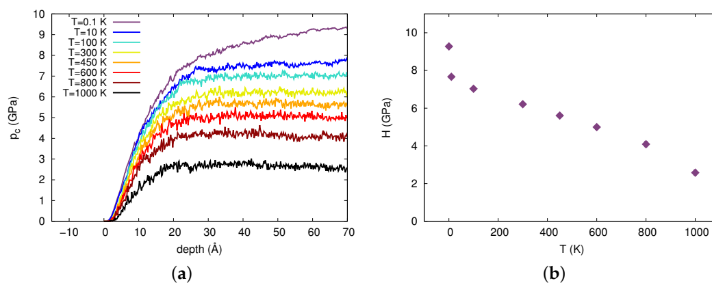
Figure 2. (a) Contact pressure as a function of indentation depth obtained for different temperatures. (b) Hardness as a function of temperature averaged from the plateau of panel (a).
