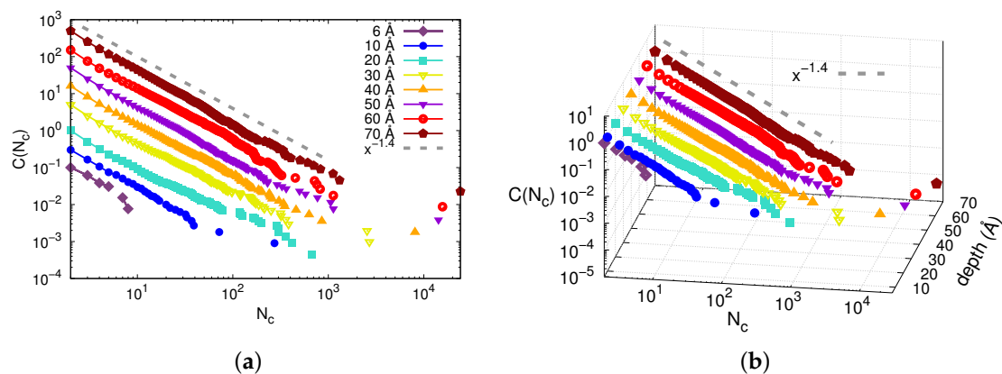
Figure 8. Complementary cumulative distributions C(N_c) at different indentation depths at T = 10 K. (a) The curves are shifted in the y direction for better readability. (b) 3D plot which avoids shifting the curves. The gray dashed line corresponds to a power law with exponent -1.4 .
