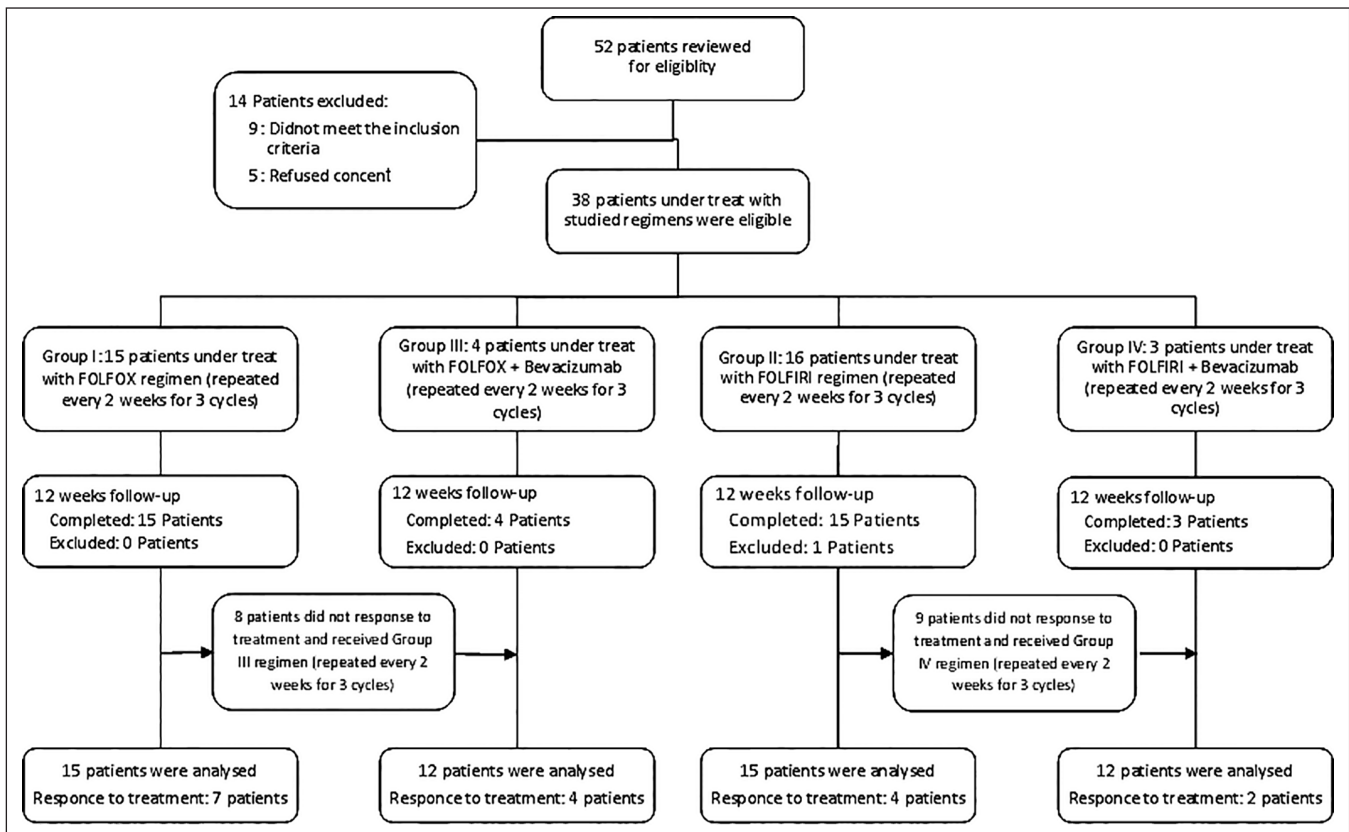
Figure 1: Study flowchart
