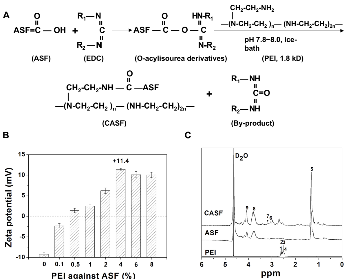
Figure 2 Synthesis and characteristics of CASF. (A) Schematic diagram of CASF synthesis. (B) Zeta potential of CASF at PEI/ASF weight ratios of 0%, 0.1%, 0.5%, 1%, 2%, 4%, 6% and 8%. (C) ^1\text{H-NMR} spectra of PEI, ASF and CASF in \text{D}_2\text{O} .
