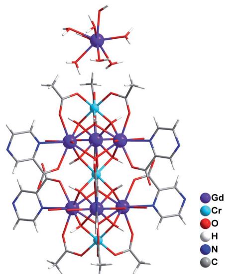
Fig. 1 Ball and stick views of the cationic cluster of \{Gd(H_2O)_8[Gd_6-Cr_3(L)_6(CH_3COO)_6(\mu_3-OH)_{12}(H_2O)_{12}]\}_6^{6+} .
