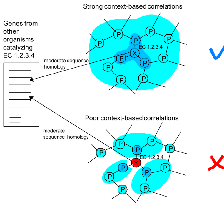
Figure 1. Illustration of the developed approach. In the figure network nodes represent metabolic genes and edges represent connections established by shared metabolites. Using sequence homology, genes X and Y from different organisms have been assigned to EC 1.2.3.4. Gene X displays strong context-based correlations (darker blue indicating stronger correlations) with neighboring network genes. Consequently, the annotation of X is likely to be correct. In contrast, gene Y does not fit well in the assigned network position and is likely to be misannotated.
