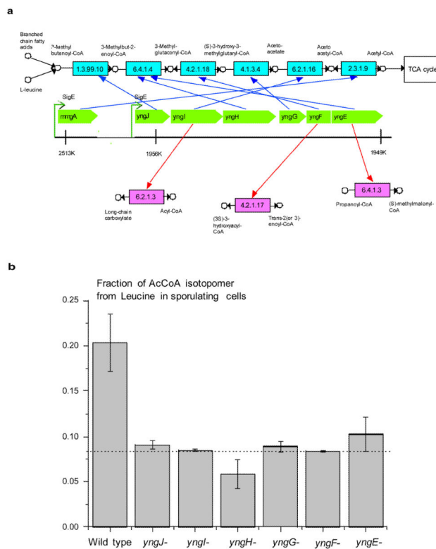
Figure 3. Function of genes forming the yng cluster in B. subtilis . a) The genomic positions of the yng genes are shown in green. The detected misannotations are indicated in red. The predicted functions, forming the degradation pathway, are shown in blue. The expression of all yng gene is controlled by the \sigma^E transcription factor 34 ; the gene mmgA is also under the \sigma^E control and is responsible for the last step of the leucine catabolism. b) Fractional ^{13}\text{C} labeling of Acetyl-CoA in the wild type sporulating cells and in the sporulating yng mutants. The ^{13}\text{C} labeling in the figure indicates the fraction of the Acetyl-CoA isotopomer generated from leucine in sporulating cells only (see Methods). The errors in the figure represent SEM. The background Acetyl-CoA isotopomer labeling is shown by the dash line.
