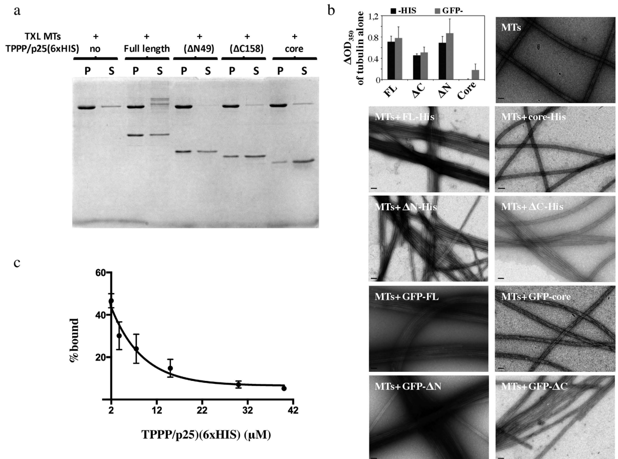
Figure 3. Microtubule binding properties of TPPP/p25. (a) Taxol stabilized microtubules ( 2\mu\text{M} ) were incubated in the presence of 2\mu\text{M} of each of the different TPPP/p25 fragments (FL, \Delta N, \Delta C and core) for 15 min before centrifugation. Coomassie-stained gel of microtubule bound and unbound TPPP/p25 fragments present in the pellets and in the supernatants, respectively. (b) Bar graph showing the changes in turbidity of tubulin solutions ( 15\mu\text{M} ) in the presence of stoichiometric amounts of the different TPPP/p25 fragments. The \text{OD}_{350} of control tubulin solutions at mass steady state were subtracted from the tubulin solutions assembled in the presence of the different TPPP/p25 fragments tagged with either 6\times\text{HIS} at their C-termini or GFP- at the N-termini. Data were compared using the Mann Whitney test (p values for the HIS- vs the GFP- tagged fragments were 1, 0,666, 0,667 and 0,333 for FL, \Delta N, \Delta C, and core respectively; p values for the FL, or \Delta N, or \Delta C fragments compared to the core were 0,028, 0,2 and 0,57, respectively; n = 4 ). EM images of taxol stabilized microtubules ( 2\mu\text{M} ) incubated with bacterially expressed and then purified C-terminal His- or GFP-tagged TPPP/p25 fragments at equimolar ratios (scale bars = 50 nm). (c) His tagged TPPP/p25 competes with GFP-tagged TPPP/p25 for MT binding. Taxol stabilized MTs were first co-incubated with 2\mu\text{M} of 6\times\text{HIS} -FL and 2\mu\text{M} GFP-FL-TPPP/p25 and then with increasing concentrations of 6\times\text{HIS} -FL. Each data point represents the mean \pm SD from three independent experiments.
