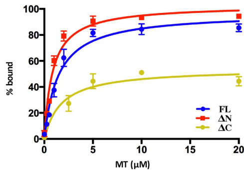
Figure 4. Quantitative analysis of the TPPP/p25 binding interaction to taxol stabilized microtubules. Binding curves with 1.5 \mu\text{M} GFP-tagged TPPP/p25 (WT or \Delta\text{N} , \Delta\text{C} ) at increasing MT concentrations. Each data point represents the mean \pm SD from three independent experiments.
