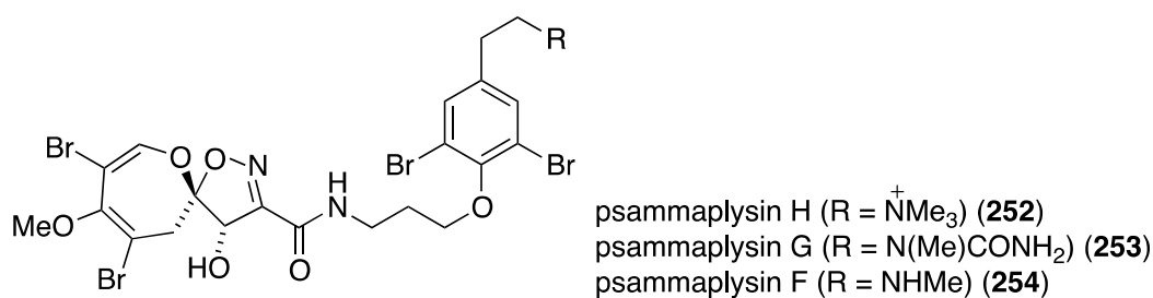
Figure 45. Structures of psammalyisins H ( 252 ), G ( 253 ), and F ( 254 ) from the sponge Pseudoceratina sp. [104].
