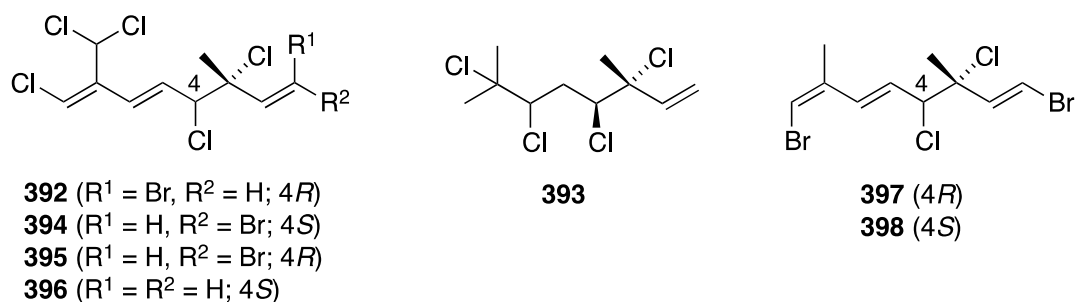
Figure 77. Structures of halogenated monoterpenes from Plocamium suhrii [156].
