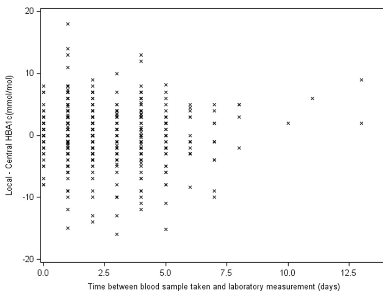
Fig. 2 Scatterplot showing the distribution of the magnitude of differences between local and central measurements by time-lag in days: between blood samples being taken and analysis at the central laboratory
