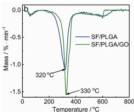
Fig. 5. TG (a) and DTG (b) curves of SF/PLGA mat and SF/PLGA/GO mat.
