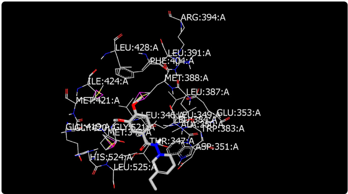
Figure 4. Docking of EH1 to ER \alpha : EH1 has a slight affinity for amino acids in the active site.
