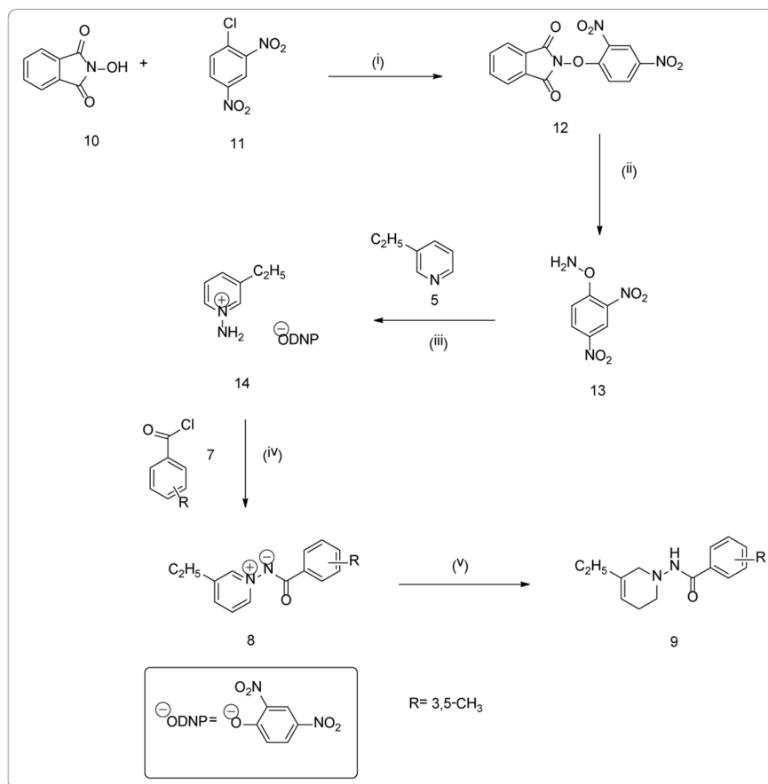
Figure 2. Scheme 2 reactions and conditions: (i) Et 3 N, 2,4-dinitrochlorobenzene, Acetone, RT, 2 h (ii) NH 2 NH 2 H 2 O, DCM:MeOH, 0°C, 8 h (iii) 3-ethylpyridine (5), MeCN, 40°C, 12 h (iv) a.) Substituted acyl chloride (7), THF, Et 3 N, 70°C, overnight b.) NaHCO 3 /H 2 O(v) NaBH 4 , abs. EtOH, 0°C, 7 h.
