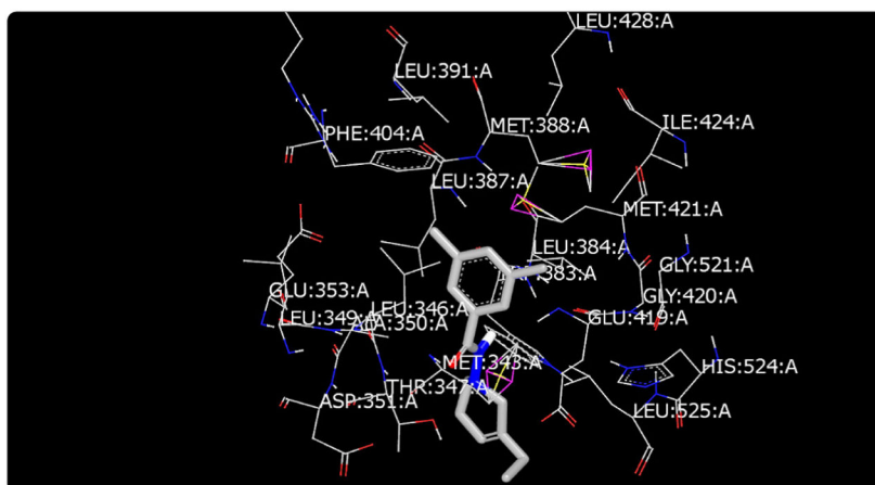
Figure 7. Docking of EH4 to ER \alpha : EH4 has a slight affinity for amino acids in the active site.
