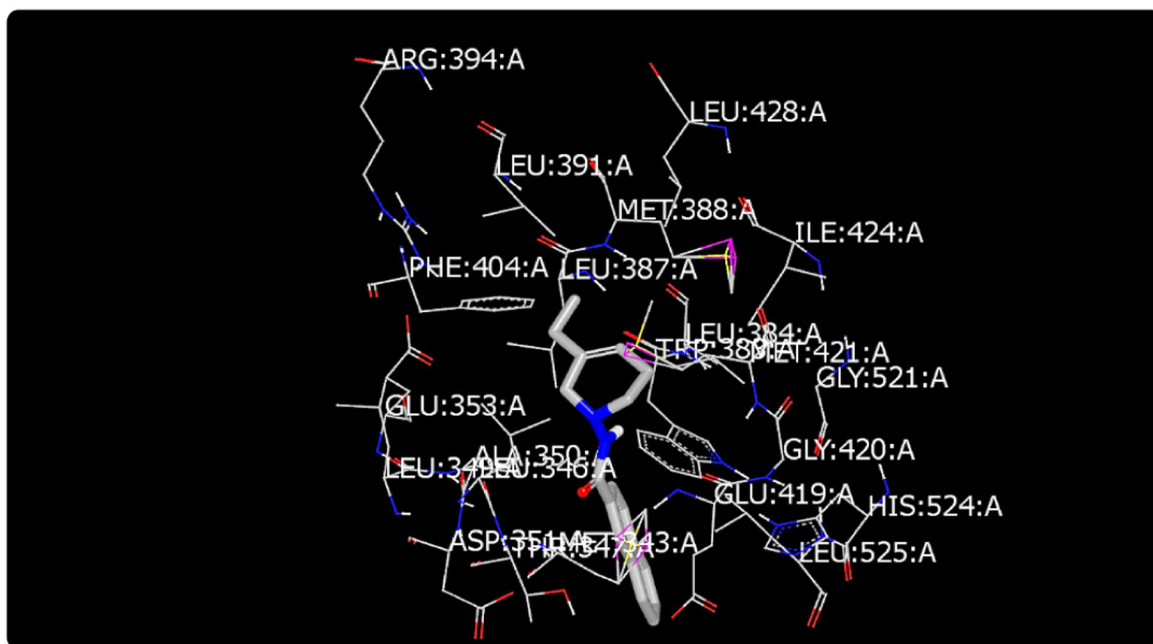
Figure 5. Docking of EH2 to ER \alpha : EH2 showed pi stacking interactions with the amino acids within the active site.
