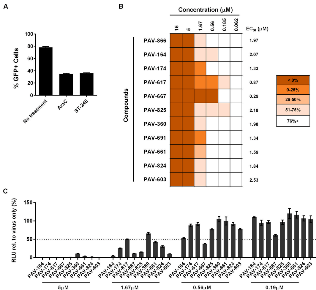
Fig. 2. Reduction in VACV spread and early gene expression by PAV-866 and derivatives(A) Percentage of GFP + cells in the presence of inhibitors AraC (DNA replication) and ST-246 (EV membrane wrapping). HeLa cells were infected with VACV-NLS-GFP at MOI 0.4 for 24 h in the absence and presence of inhibitors. Samples were fixed and stained with DAPI to visualize total number of cells. The percentage of infected cells was determined as the ratio of GFP + nuclei to total number of nuclei. Values represent the mean of two or more replicates±SEM. (B) Percent VACV spread in the presence of serially diluted PAV-866 and derivatives. Shading of cells corresponds to degree of viral inhibition (darkest cells indicate low viral spread or high viral inhibition). Corresponding EC 50 values also shown. (C) HeLa cells were infected with VACV-LUC virus at MOI 3 in the presence or absence of four concentrations of 10 PAV-866 analogs. After 2 h, cells were lysed and luciferase activity was measured as a surrogate for early gene expression. The values plotted represent the percent relative luminescence units (RLU) of each treatment with respect to cells infected with virus alone. The dotted line represents the 50% RLU value relative to the virus only treatment. The mean of two or more replicates is shown±SEM.
